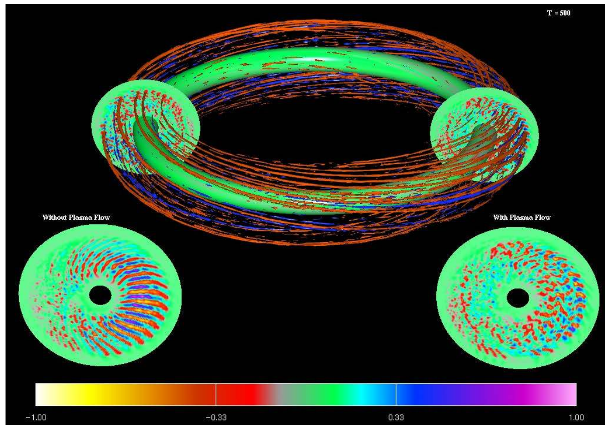
Figure 4. Comparison of nonlinear mode structure: effects of zonal flows. GTC simulations, Gyrokinetic Toroidal Code (GTC) ® Princeton plasma physics laboratory. http://w3.pppl.gov/theory/bin/zonal-flow.jpg
