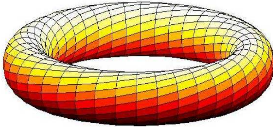
Figure 3. Gyrokinetic particle simulation. Implementation of Mixed-Mode Parallelism ® Princeton plasma physics laboratory. http://w3.pppl.gov/theory/proj_gksim.html
