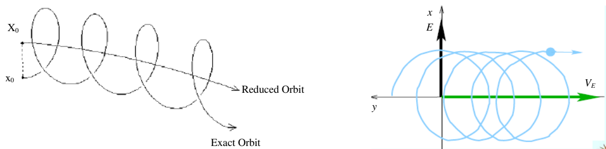
Figure 2. Exact and reduced single-particle orbits in a magnetic field. [5] [7].
