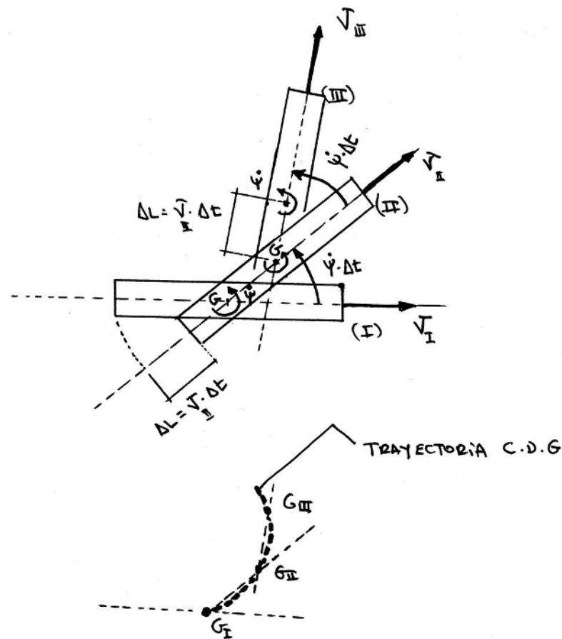
Figure 6. The position of the center of mass varies depending on the coupling between the field of the linear velocity and the velocity field caused by the non-coaxial torque [35]. (Figure Alejandro Alvarez).
