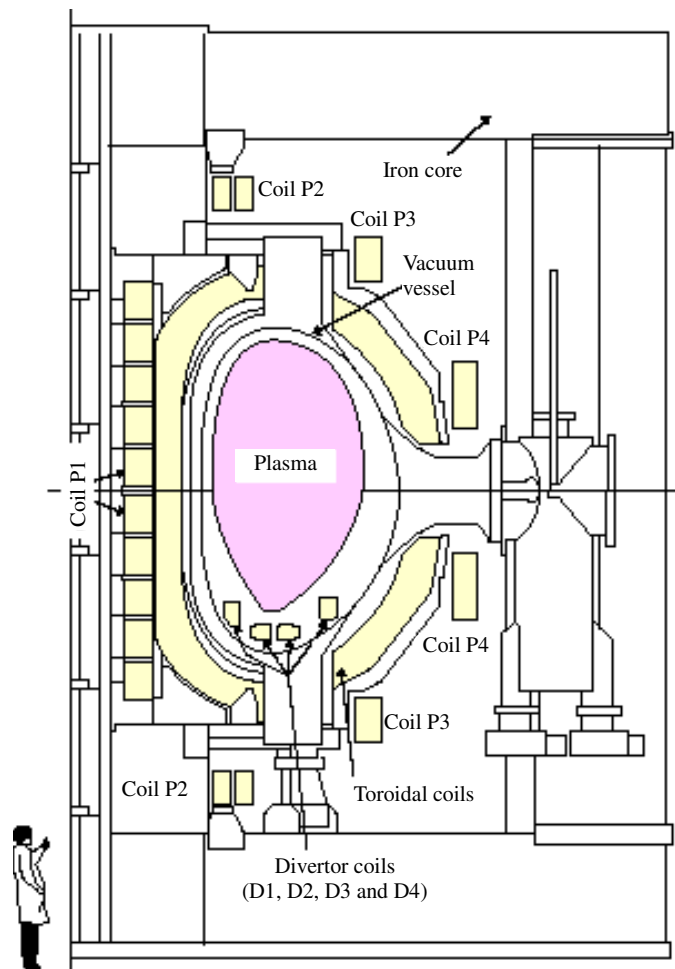
Figure 1. Joint European torus (European fusion development agreement—EFDA).
