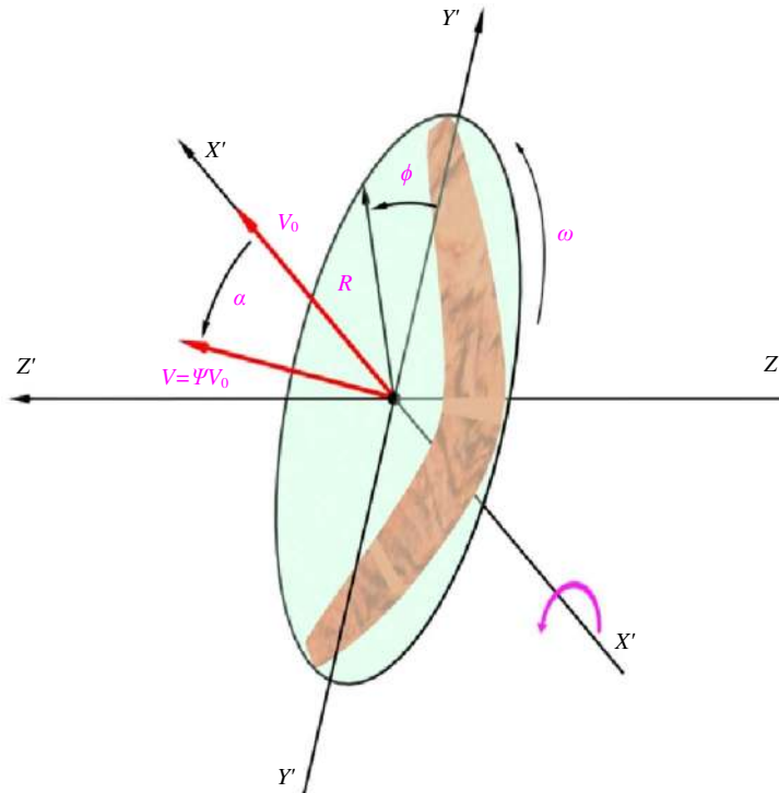
Figure 5. Rotations that generate changes in the boomerang’s path as a result of the coupling of the velocity fields that act on its center of mass [28].
