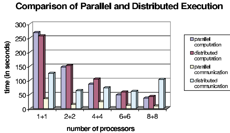
Fig. 3. Comparison of parallel and distributed execution.
