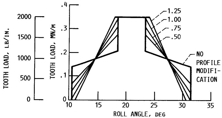
(b) SHARED TOOTH LOAD.
