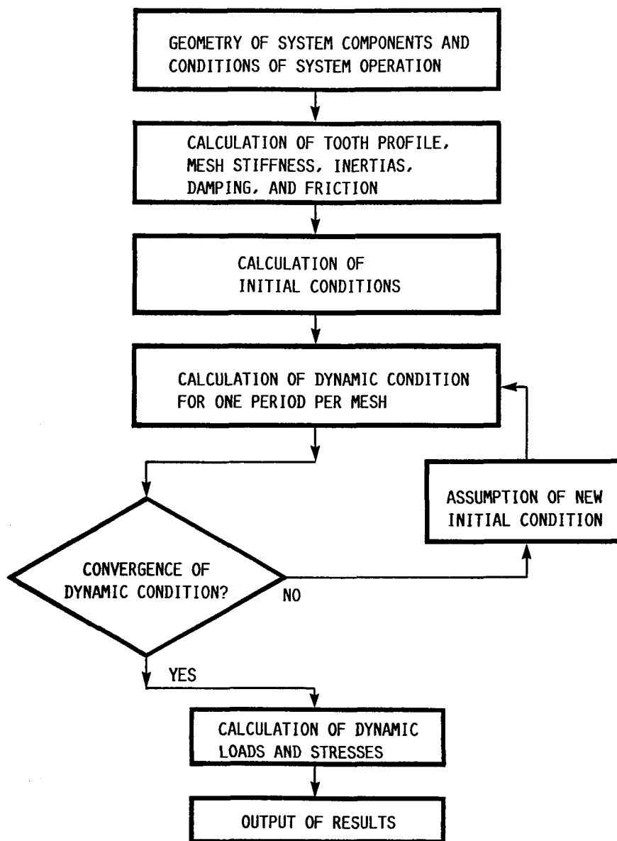
FIGURE 2. - FLOW CHART OF COMPUTATIONAL PROCEDURE.
