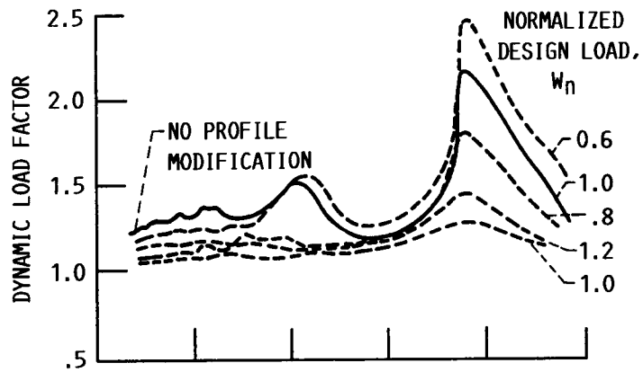
(a) DYNAMIC LOAD FACTOR.
