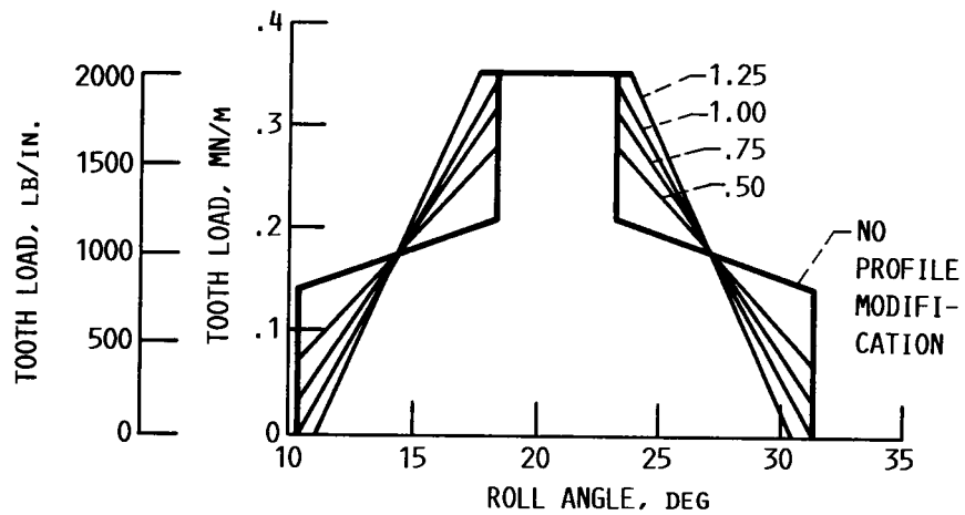
(b) SHARED TOOTH LOAD.
