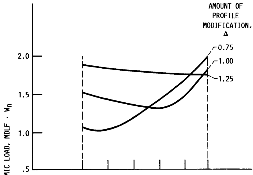
(a) LINEAR PROFILE MODIFICATION.
