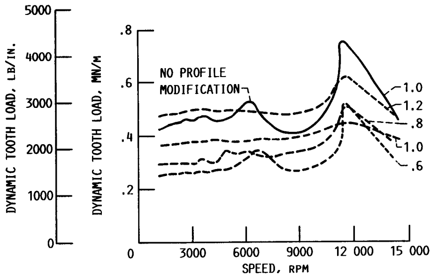
(b) TOTAL DYNAMIC TOOTH LOAD.
