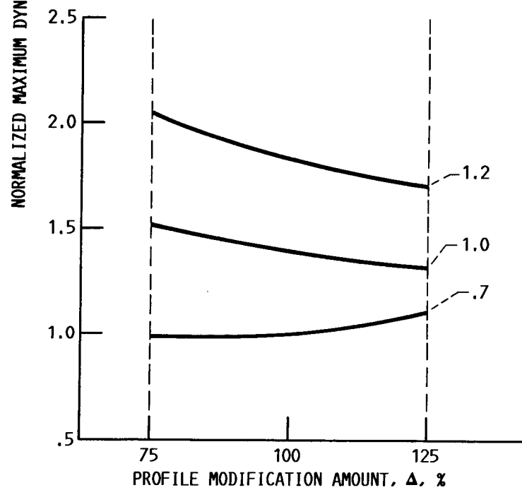
(b) PARABOLIC PROFILE MODIFICATION.
