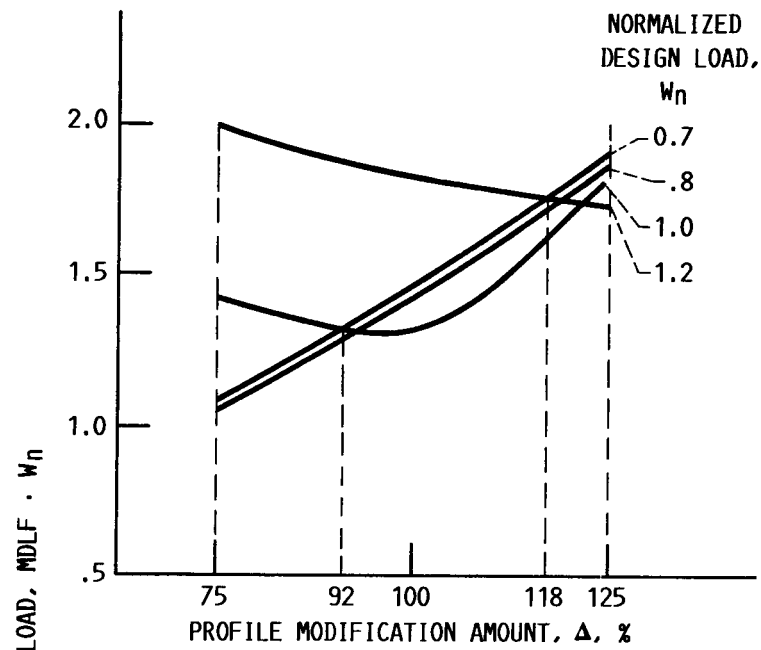
(a) LINEAR PROFILE MODIFICATION.
