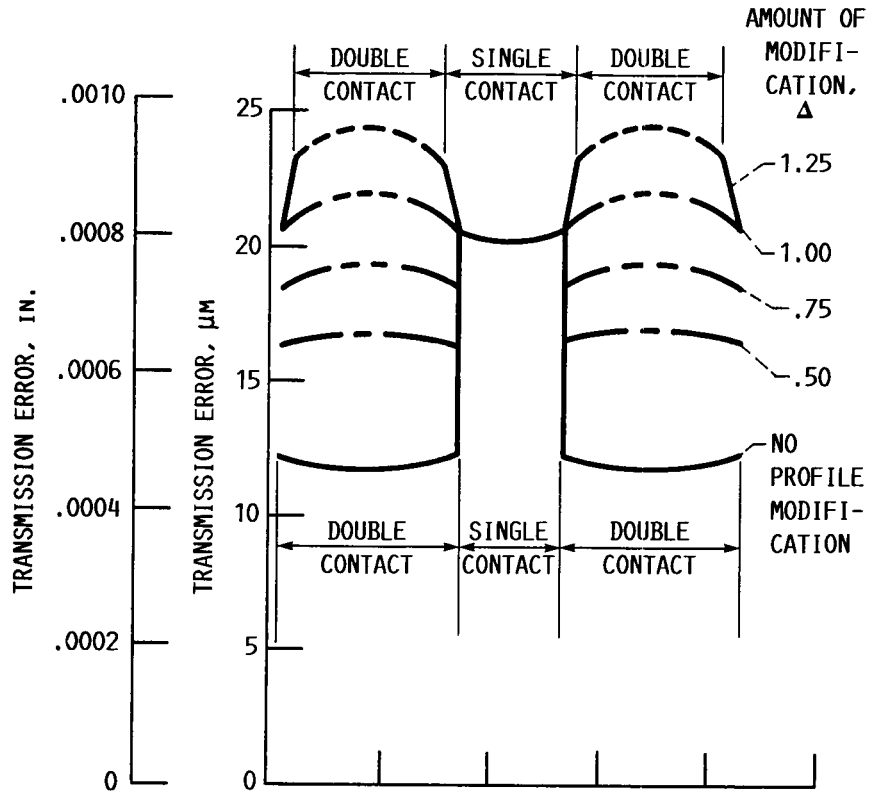
(a) STATIC TRANSMISSION ERROR.
