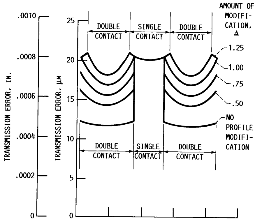
(a) STATIC TRANSMISSION ERROR.
