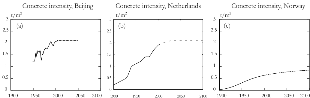
Figure 9 Historical figures and projections of the concrete intensity (tonnes per square meter floor area [ t/m^2 ]) in housing construction in Beijing, China; the Netherlands (medium scenario); and Norway (medium scenario). One tonne ( t ) = 10^3 kilograms (kg, SI) \approx 1.102 short tons. Source: Liu and Hu 2006; BMBS 1999, 2000–2007; Müller 2006; Bergsdal et al. 2007a
