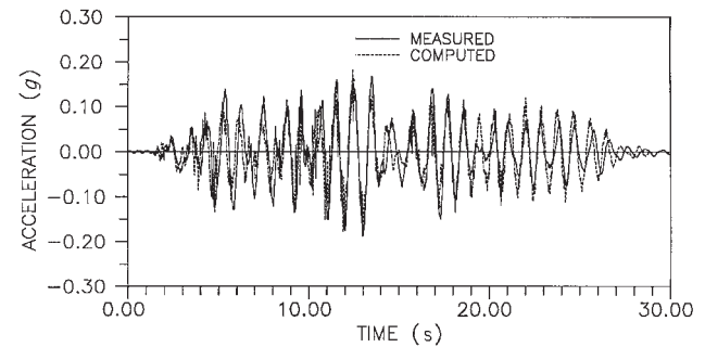
Fig. 7. The computed versus measured acceleration response at the pile head of the single pile.
