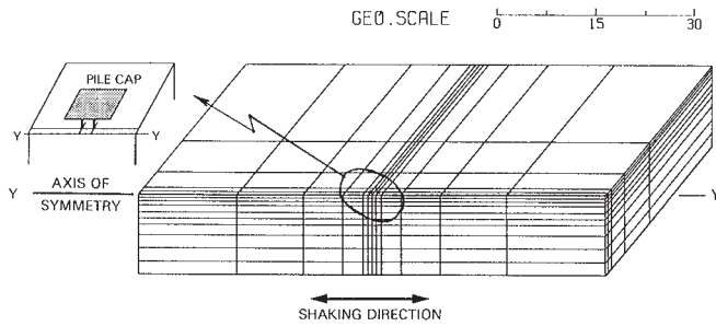
Fig. 11. Finite element modelling of the four-pile group.
