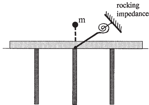
Fig. 2. A mechanical model used for the analysis of a pile group with a rigid pile cap.
