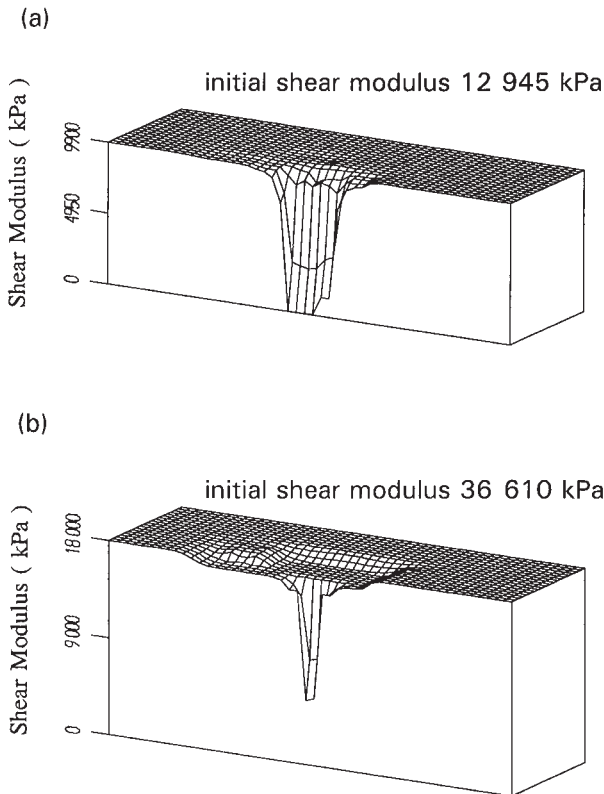
Fig. 16. Three-dimensional plots of the distribution of shear moduli at t = 12.58 s from the single pile analysis: (a) at a depth of 0.25 m, and (b) at a depth of 2.10 m.
