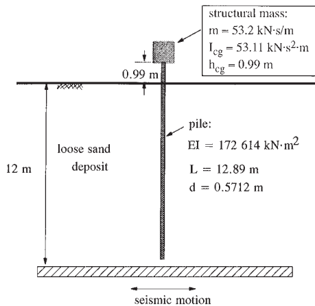
Fig. 4. The prototype model of the single pile test.
