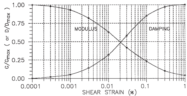
Fig. 6. The relationships between shear modulus, damping, and the shear strain for the loose sand.
