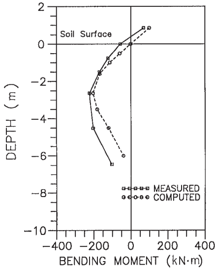
Fig. 15. Comparison between measured and computed bending moments at peak pile cap displacement for the four-pile group.
