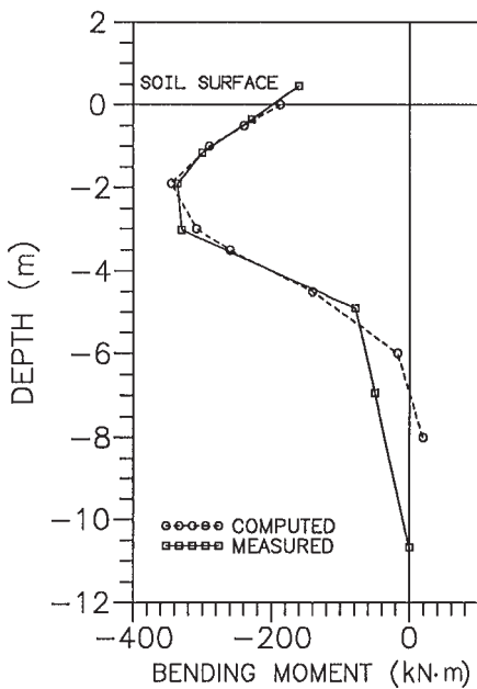
Fig. 9. Comparison between measured and computed bending moments at peak pile deflection for the single pile.
