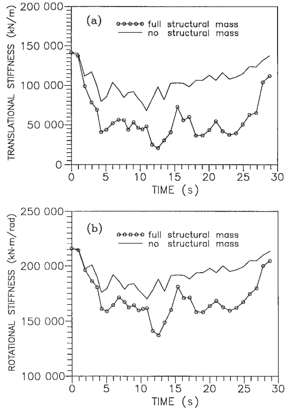
Fig. 20. Comparison of dynamic stiffnesses of the single pile with and without structural mass: (a) translational stiffness k_{vv} (b) rotational stiffness k_{\theta\theta} .
