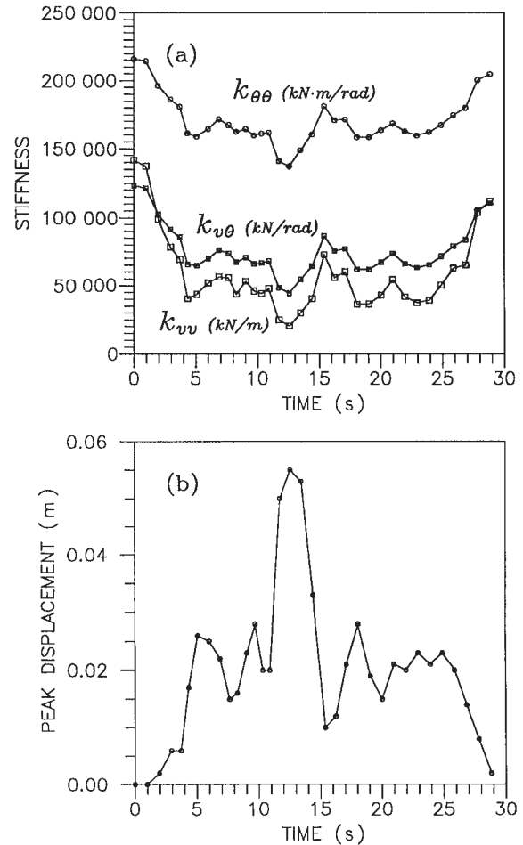
Fig. 17. Variation with time of (a) pile head stiffnesses k_{vv} , k_{v\theta} , and k_{\theta\theta} at f = 1.91 Hz and (b) peak pile head displacements.
