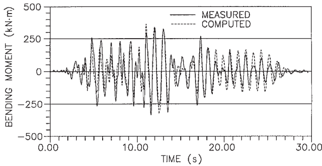
Fig. 8. The computed versus measured moment response at depth D = 3 m of the single pile.
