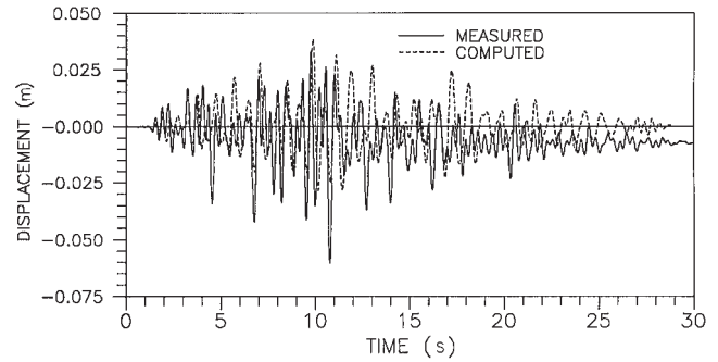
Fig. 13. The computed versus measured displacement response at the top of structural mass of the four-pile group.
