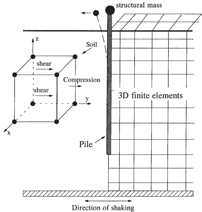
Fig. 1. The principle of the quasi-3D dynamic analysis of the pile-soil-structure interaction.
