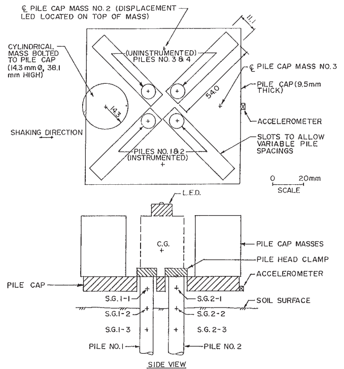
Fig. 10. Layout of centrifuge test for a four-pile group.
