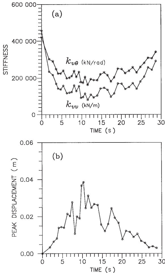
Fig. 19. Variation with time of (a) stiffnesses k_{vv} and k_{v\theta} of the four-pile group at f=1.91 Hz, and (b) peak displacements at the pile cap.
