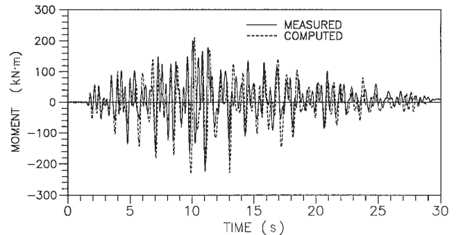
Fig. 14. The computed versus measured moment response at depth D = 2.63 m of the four-pile group.
