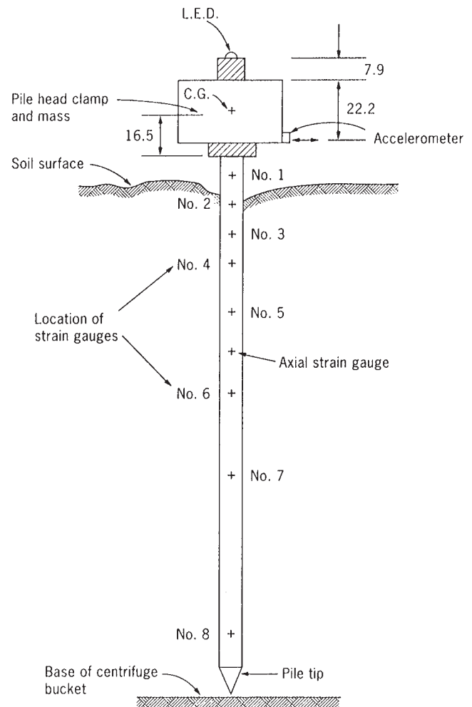
Fig. 3. The layout of the centrifuge test for a single pile. C.G., centre of gravity; L.E.D., light emitting device.
