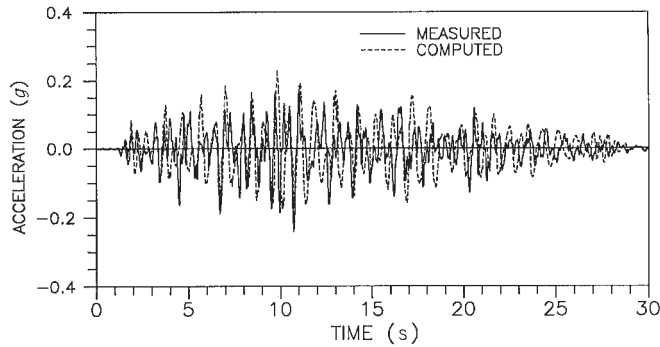
Fig. 12. The computed versus measured acceleration response at the pile cap of the four-pile group.
