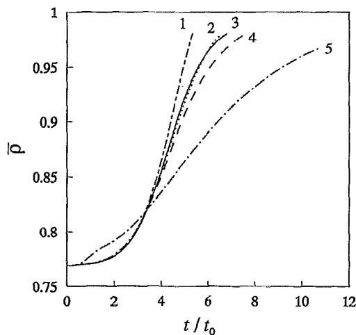
FIG. 6. Effect of strain hardening and thermal softening on dynamic pore collapse of an elastic/viscoplastic aluminum spherical shell: a_0=20 \mu\text{m} , \bar{\rho}_0=0.769 , \dot{p}=10 \text{ MPa/ns} , \tau=\tau_0(\dot{\gamma}/\dot{\gamma}_0)^m(\gamma/\gamma_0)^n(\theta/\theta_0)^v , and t_0=21.65 \text{ ns} : (1) n=0 , v=-1.0 ; (2) n=0.04 , v=-0.4 ; (3) n=v=0 ; (4) n=0.04 , v=0 ; (5) n=0.25 , v=0 .
