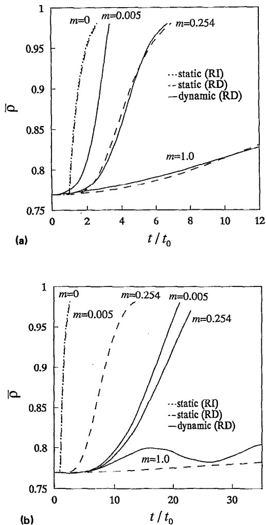
FIG. 4. Comparison of static and dynamic pore collapse of an elastic/viscoplastic aluminum spherical shell of initial pore radius a_0=20\ \mu\text{m} and initial relative density \bar{\rho}_0=0.769 . The material model for plastic deformation in the current dynamic analysis is given as \tau=\tau_0(\dot{\gamma}/\dot{\gamma}_0)^m : (a) With an applied external pressure rate \dot{p}=10\ \text{MPa/ns} , t_0=21.65\ \text{ns} ; (b) with an applied external pressure rate \dot{p}=250\ \text{MPa/ns} and t_0=0.866\ \text{ns} .
