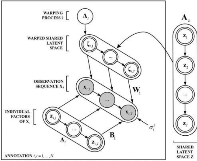
Fig. 2. Graphical model of DPCTW. Shaded nodes represent the observations. By ignoring the temporal dependencies, we obtain the PCTW model.
