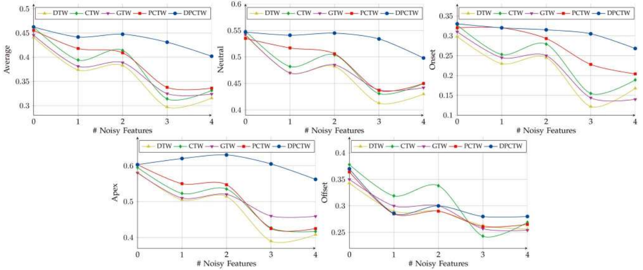
Fig. 8. Accuracy of DTW, CTW, GTW, PCTW and DPCTW on the problem of action unit alignment under spiked noise added to an increasing number of features for AU = 12 (smile).
