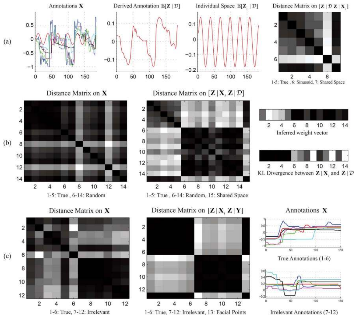
Fig. 7. Annotation filtering and ranking (black - low, white - high). (a) Experiment with a structured false annotation (sinusoid). The shared space is not affected by the false annotation, which is isolated in the individual space. (b) Experiment with 5 true and 9 spammer (random) annotations. (c) Experiment with 6 true annotations, 7 irrelevant but correlated annotations (belonging to a different sequence). The facial points Y , corresponding to the 6 true annotations, were used for supervision (with SG-DPCCA).
