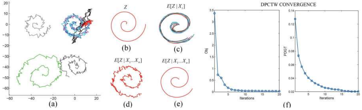
Fig. 4. Noisy synthetic experiment. (a) Initial, noisy time series. (b) True latent signal from which the noisy, transformed spirals were attained in (a). (c) Alignment achieved by DPCTW. The shared latent space recovered by (d) PCTW and (e) DPCTW. (f) Convergence of DPCTW in terms of the objective (Obj) (Eq. 17) and the path difference between the estimated alignment and the true alignment path (PDGT).
