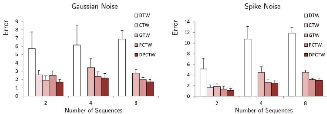
Fig. 5. Synthetic experiment comparing the alignment attained by DTW, CTW, GTW, PCTW and DPCTW on spirals with spiked and Gaussian noise.
