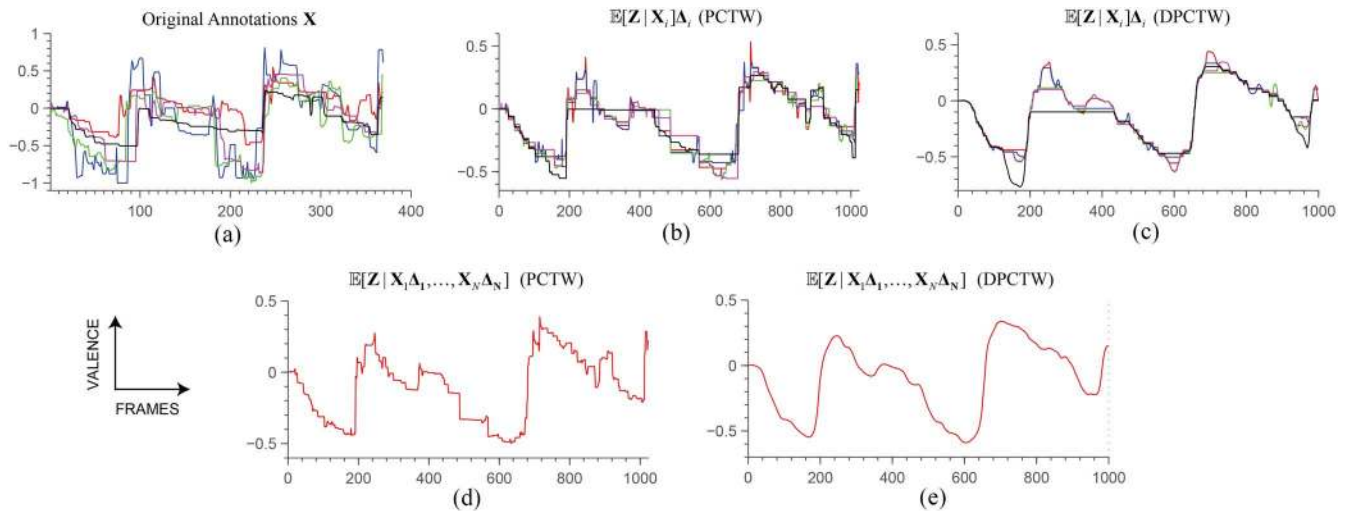
Fig. 6. Applying (D)PCTW to continuous emotion annotations. (a) Original valence annotations from 5 experts. (b, c) Alignment obtained by PCTW and DPCTW respectively, (d, e) Shared space obtained by PCTW and DPCTW respectively, which can be considered as the “derived ground truth”.
