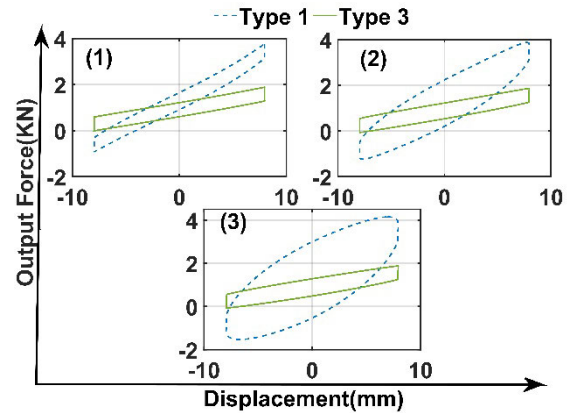
FIGURE 6. The comparison of Type 1 IC HPS and Type 3 IC HPS at Out-of-phase test. Note: the number in figures is similar those listed in Table 4.
