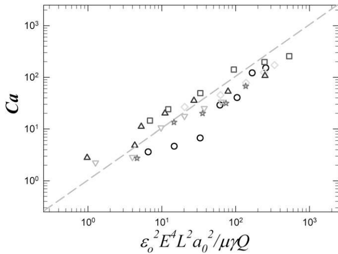
Fig. 5. A log–log plot of the capillary number Ca \approx \mu Q / \gamma a_{0min}^2 versus \varepsilon_0^2 E^4 L^2 a_0^2 / \mu \gamma Q for the transition to coiling. The grayscale symbols correspond to different experimental parameters: circles ( \circ ) ( L = 11.4 mm, Q = 30 mL/h, a_0 = 0.92 mm, \gamma = 32 mN/m); triangles-down ( \nabla ) ( L = 12.7 mm, Q = 40 mL/h, a_0 = 0.92 mm, \gamma = 32 mN/m); squares ( \square ) ( L = 8.2 mm, Q = 1 mL/h, a_0 = 0.92 mm, \gamma = 2 mN/m); diamonds ( \diamond ) ( L = 9.6 mm, Q = 0.5 mL/h, a_0 = 0.92 mm, \gamma = 2 mN/m); triangles-up ( \triangle ) ( L = 12.8 mm, Q = 10 mL/h, a_0 = 0.92 mm, \gamma = 32 mN/m); and stars ( \star ) ( L = 7.4 mm, Q = 8 mL/h, a_0 = 0.46 mm, \gamma = 32 mN/m). The data points from the same symbols correspond to different applied electric field strengths. All symbols collapse onto a dashed line representing a linear relationship, confirming our scaling relationship \varepsilon_0^2 E^4 L^2 a_0^2 / \mu \gamma Q \approx Ca , as stated in Eq. 4.
