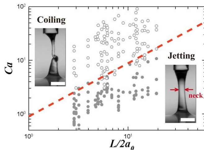
Fig. 2. A log–log state diagram showing the jetting and coiling of electrified liquid filaments, based on the capillary number Ca = \mu U_{max}/\gamma at the neck and the relative separation between the nozzle and the substrate, L/2a_0 . The state diagram contains more than 150 individual measurements and is highly reproducible. The diagram is divided into two regimes: (i) jetting, closed circles; and (ii) coiling, open circles ( Left and Right Insets are microscope images showing coiling and straight jets, respectively). (Scale bar: 2 mm.) The dashed line represents a linear relationship Ca = \mu U_{max}/\gamma \approx L/2a_0 . Here L/2a_0 is in the range of 4 to 20, fulfilling the assumption of a slender jet (36).
