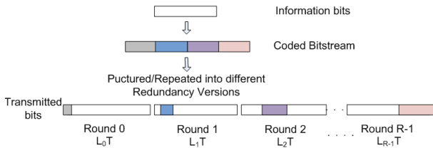
Fig. 1. Coding Model
