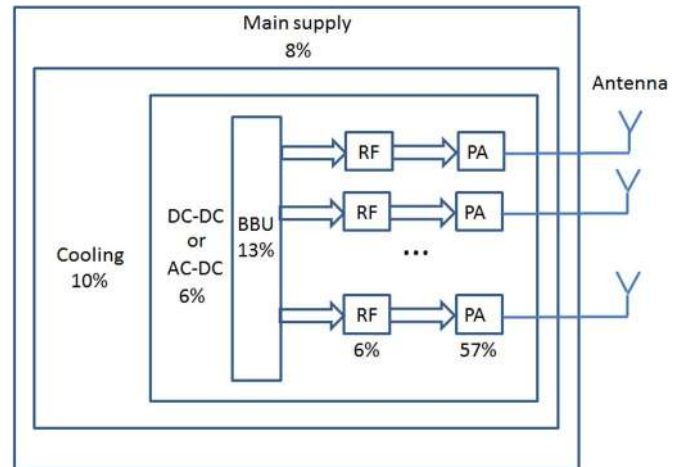
Fig. 2. Components of a BS and their power consumption percentages.
