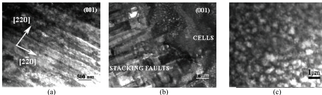
Figure 4. (a) Twins/laths at 59 GPa; (b) Dislocation cells and stacking faults at 24 GPa; (c) Dislocation cells at 18 GPa.
