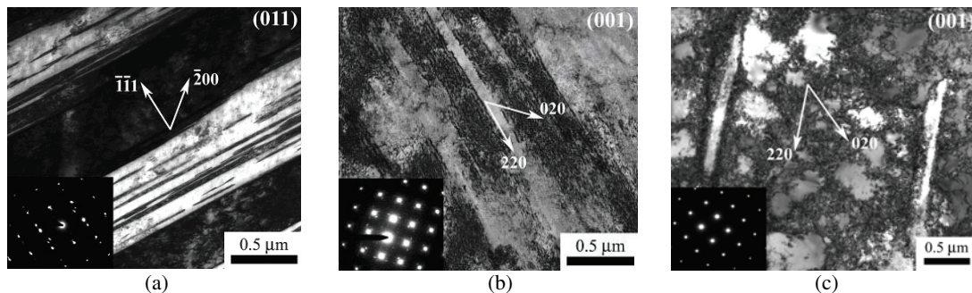
Figure 3. (a) Twinned regions \sim 0.1 mm from surface, 52 GPa.; (b) Stacking faults at 1.3 mm running along [220] , 26 GPa.; (c) Elongated and regular cells at 0.13 mm, 18 GPa.
