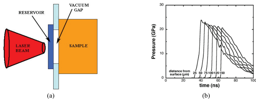
Figure 2. a) Schematic of the laser ICE setup; b) Typical pressure vs. time profile obtained, ( \sim 24 GPa).
