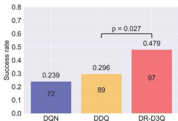
Figure 6: The human evaluation results of DQN, DDQ(20), and DR-D3Q(20) in the noisy settings. The number of dialogues is indicated on each bar and the one-sided p-value is from a two-sample permutation test (difference in mean is significant with p < 0.05 ).
