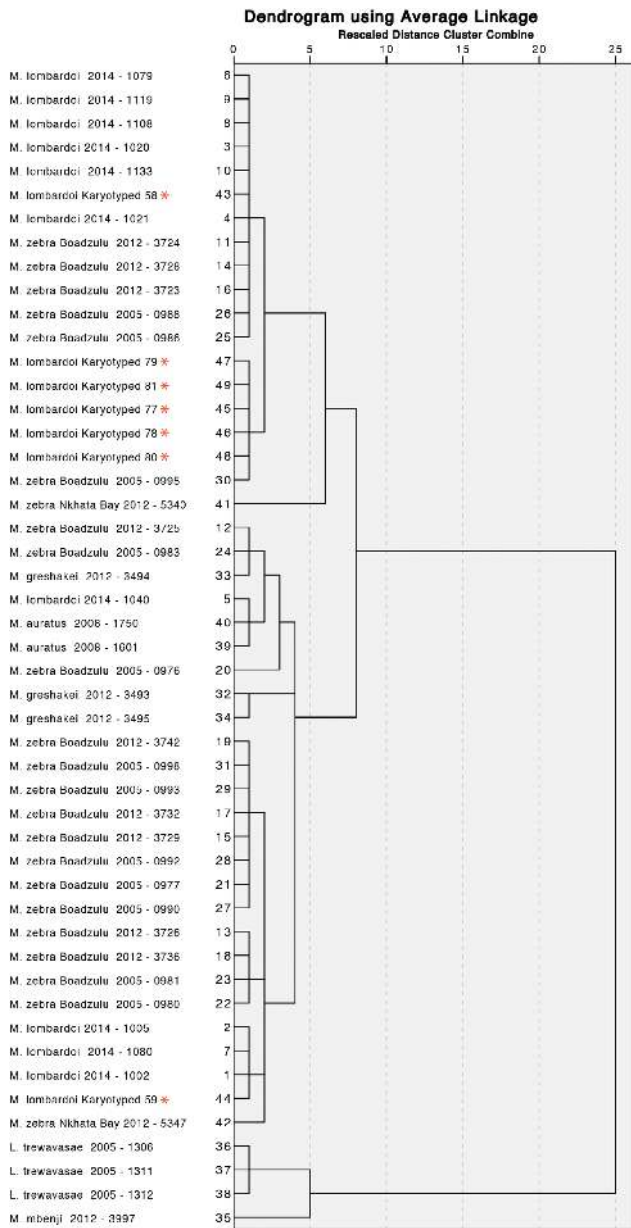
Figure 6. Cluster analysis dendrogram. Hierarchical clustering of samples by the CNVs of sequences Seq13, Seq14, Seq23, Seq32, and Seq58. Species and sample ID listed to the left. Karyotyped Metriaclima lombardoi individuals, known to have 1 B chromosome, are marked with a red asterisk (*).
