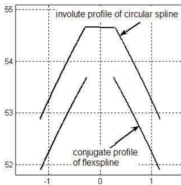
Figure 1. The theoretical conjugate tooth profile of flexspline.
