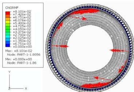
Figure15. The circumferential load distribution of un-optimized flexspline tooth
