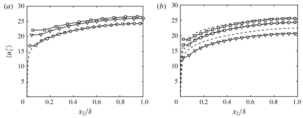
Figure 9. Effect of (a) the grid resolution and (b) Reynolds number on the mean velocity profile for I_i = 0.008\delta : (a) \Delta/\delta = 0.050 ( \circ ), 0.077 ( \nabla ), and 0.100 ( \square ); (b) Re_\tau \approx 950 ( \nabla ), Re_\tau \approx 2000 ( \circ ), Re_\tau \approx 4200 , ( \square ). DNS (dashed line).
