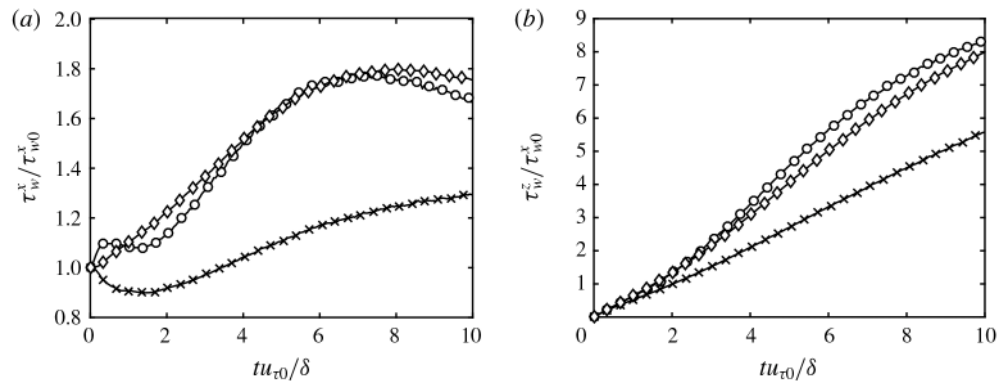
Figure 15. Wall stress in (a) streamwise and (b) spanwise directions as a function of time for the WSIM (O), EQWM (◇) and NS (x).
