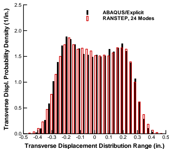
Figure 14: Mid-span transverse displacement response PDF at 35°F and 170 dB.
