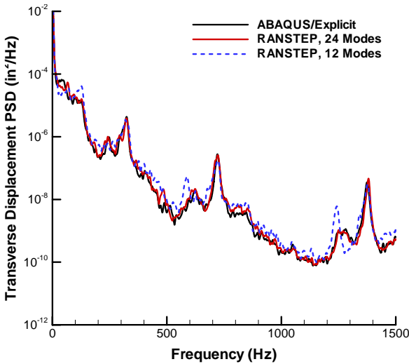
Figure 6: Mid-span transverse displacement response PSD at 35°F and 158 dB.
