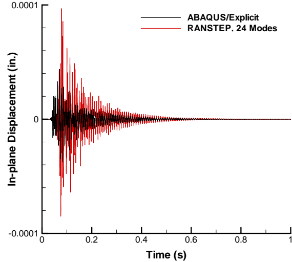
Figure 3: In-plane displacement response of a dynamic thermal buckling event.
