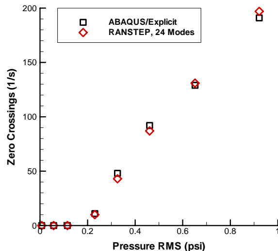
Figure 15: Transverse displacement zero-crossing intensity at 35°F.
