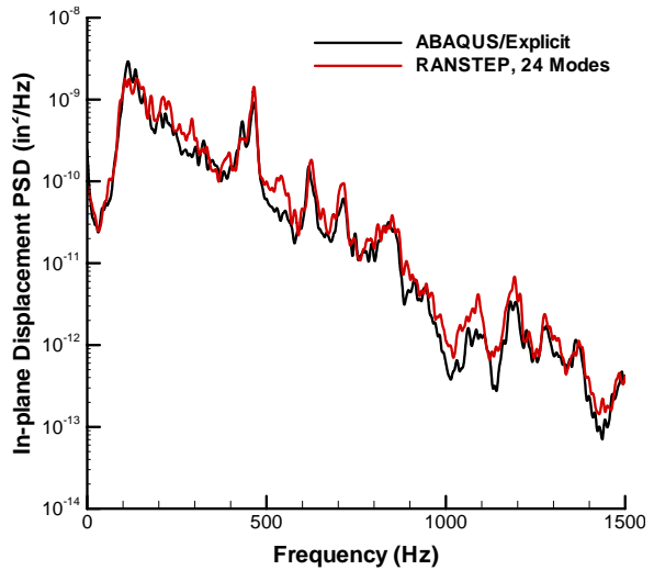
Figure 7: Mid-span in-plane displacement response PSD at 35°F and 158 dB.
