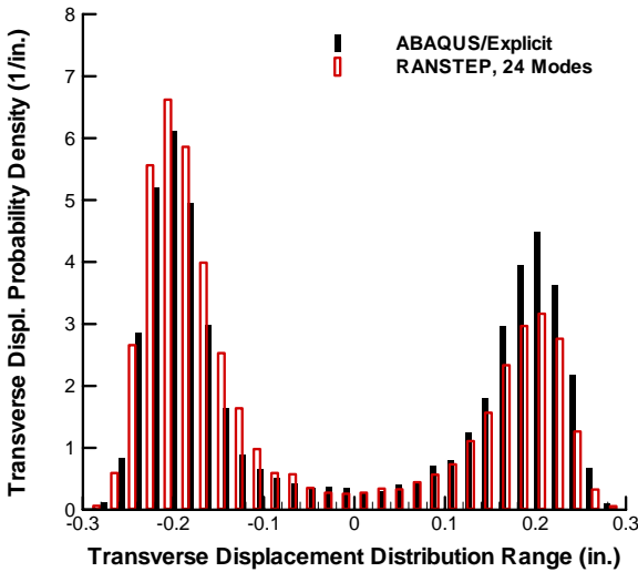
Figure 8: Mid-span transverse displacement response PDF at 35^\circ\text{F} and 158 dB.
