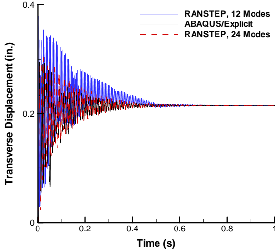
Figure 2: Transverse displacement response of a dynamic thermal buckling event.
