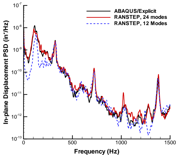
Figure 10: Quarter-span in-plane displacement response PSD at 35^\circ\text{F} and 158 dB.
