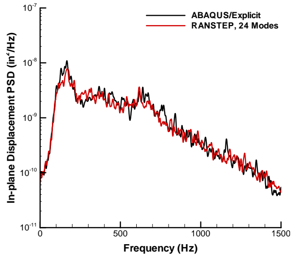
Figure 13: Mid-span in-plane displacement response PSD response at 35°F and 170 dB.
