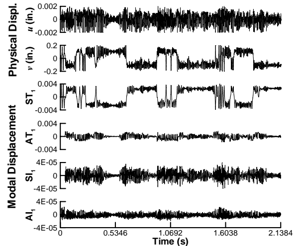
Figure 11: Quarter-span physical and modal displacement response at 35^\circ\text{F} and 158 dB.
