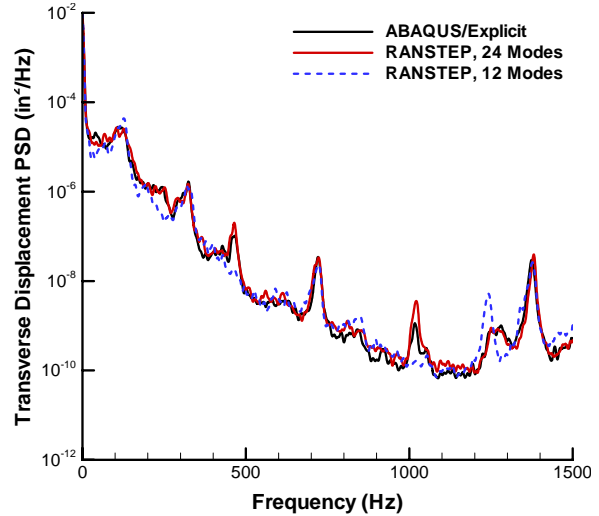
Figure 9: Quarter-span transverse displacement response PSD at 35^\circ\text{F} and 158 dB.
