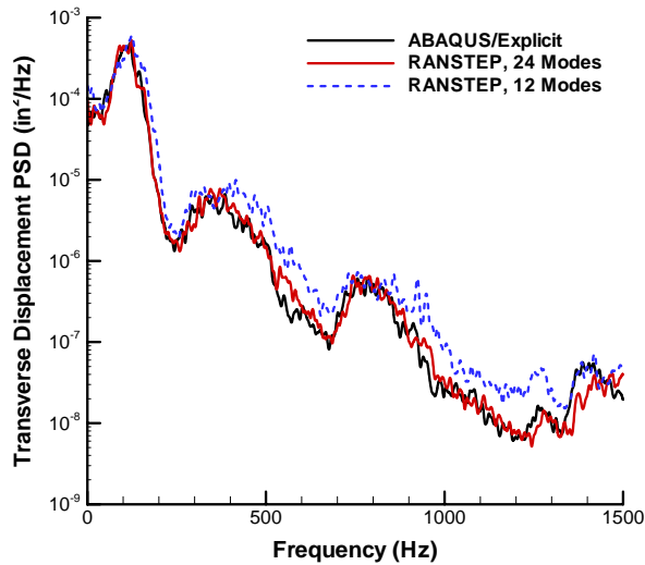
Figure 12: Mid-span transverse displacement response PSD response at 35°F and 170 dB.
