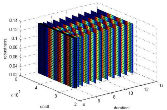
Fig. 10. Slice plot of the 50 percent-summary attainment surface obtained at the scheduling point t_i = 2.6 in Real_3 .
