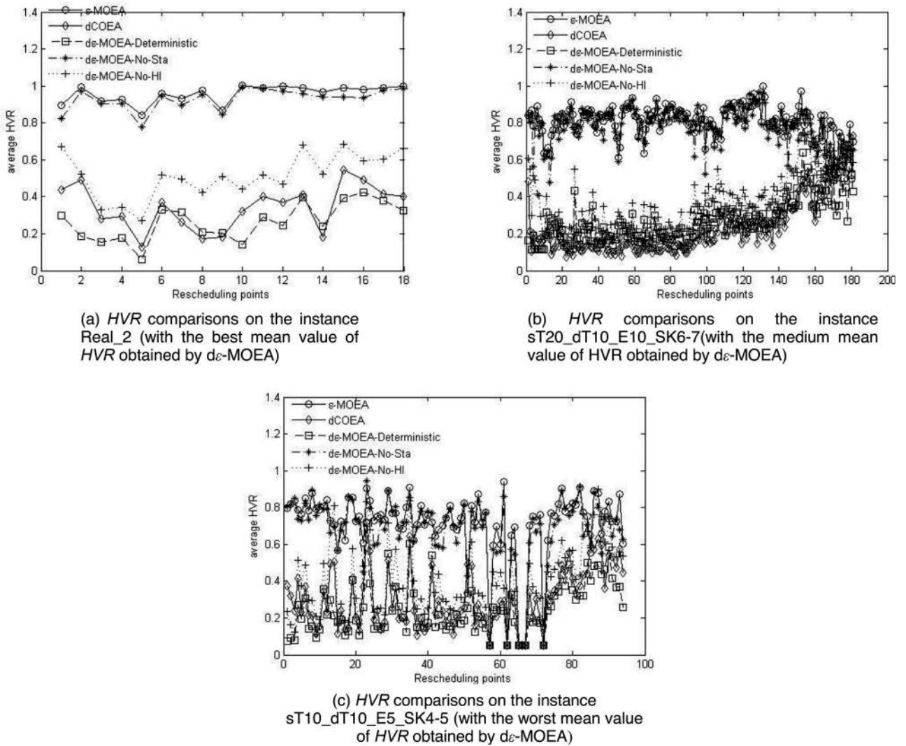
Fig. 8. Average HVR comparisons of the five methods at each scheduling point on the MODPSP instance ( HVR is to be maximized).
