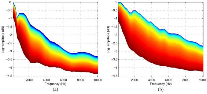
Fig. 3. Frequency profile of the prototype envelopes corresponding to two of the curves in Fig. 2. (a) Clarinet. (b) Violin.
