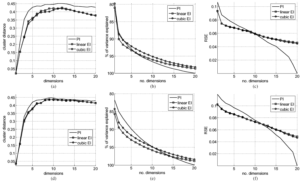
Fig. 1. Evaluation of the representation stage: results for the piano [Fig. 1(a)–(c)] and the violin [Fig. 1(d)–(f)]. Note that the y -axes of the explained variance graphs have been inverted so that for all measures, “better” means downwards. (a) Piano: train/test cluster distance (representativeness criterion). (b) Piano: explained variance (compactness criterion). (c) Piano: RSE (accuracy criterion). (d) Violin: train/test cluster distance (representativeness criterion). (e) Violin: explained variance (compactness criterion). (f) Violin: RSE (accuracy criterion).
