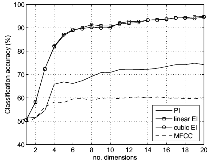
Fig. 6. Isolated sample classification results: Averaged classification accuracy.
