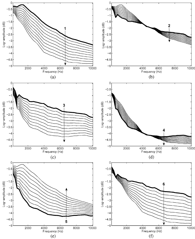
Fig. 5. Evolution of the spectral envelope alongside the traces in Fig. 4. (a) Trace 1. (b) Trace 2. (c) Trace 3. (d) Trace 4. (e) Trace 5. (f) Trace 6.
