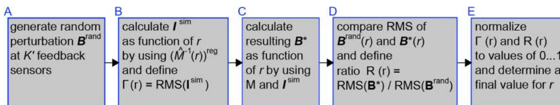
FIG. 8. Flow-chart of the process used to optimize the regularization parameter.
