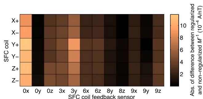
FIG. 14. Absolute value of the difference between regularized \hat{M}_{jk}^{-1} and non-regularized \hat{M}_{jk}^{-1} pseudoinverse of the proportionality matrix M for the set of twelve feedback sensors used in the tests. The value of the difference increases with increasing effect of regularization on the specific matrix element. Sensor 0x shows the largest effect.
