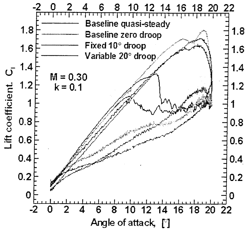
Fig. 11: Lift coefficient integrated from measured pressure distributions.
