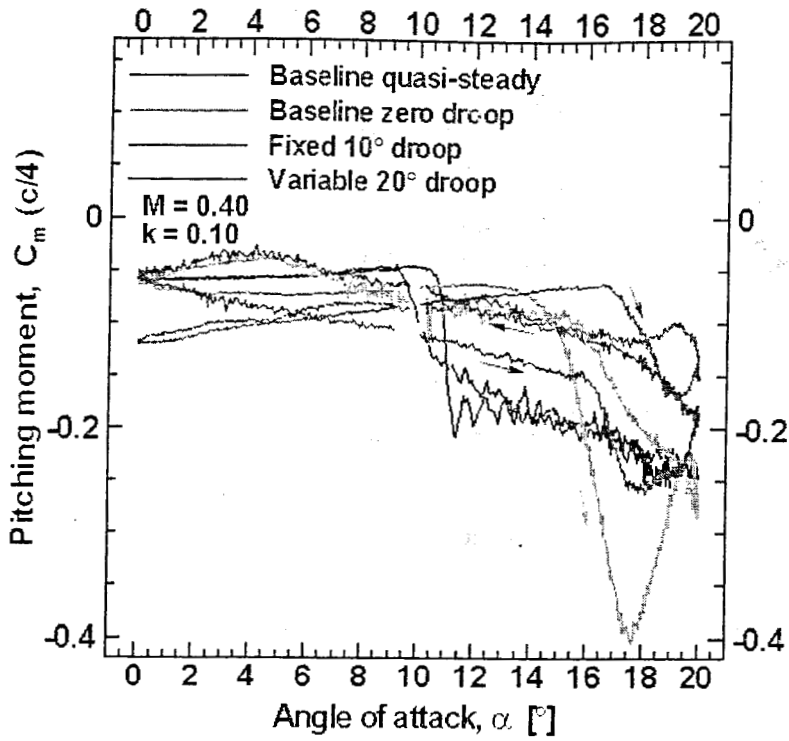
Fig. 19: Moment coefficient integrated from measured pressure distributions.
