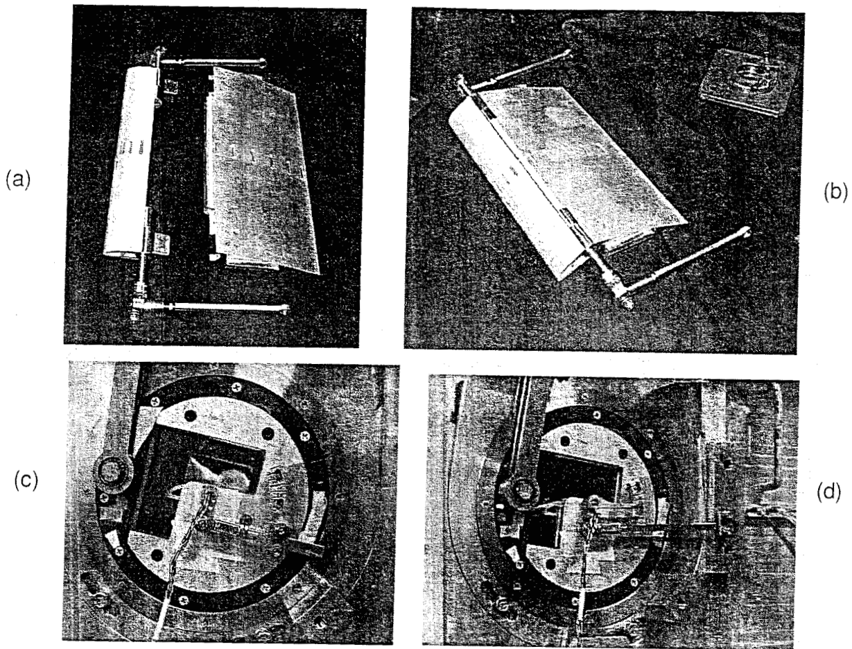
Fig. 3. VDLE airfoil and wind tunnel mounting configurations.
