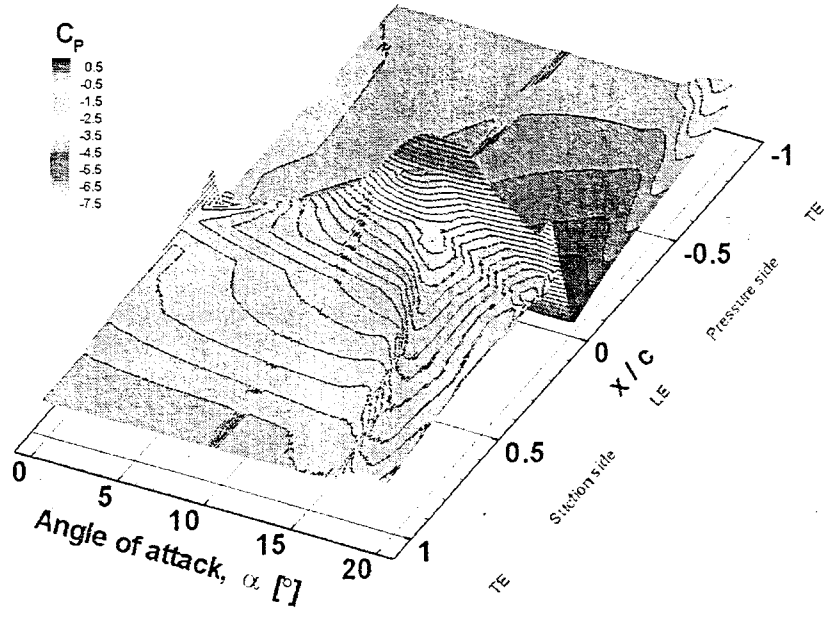
Fig. 15: Pressure contours during the upstroke
