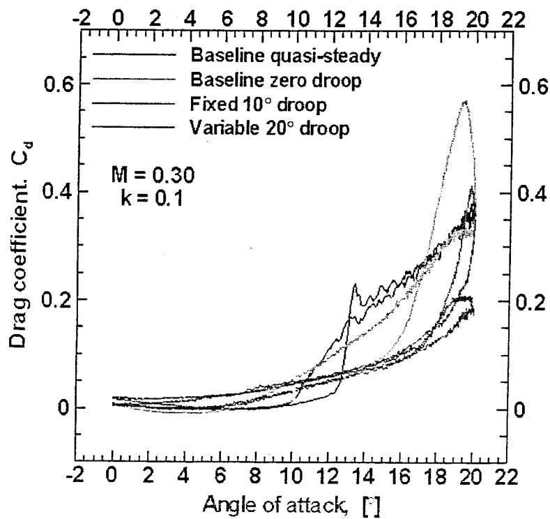
Fig. 12: Drag coefficient integrated from measured pressure distributions.
