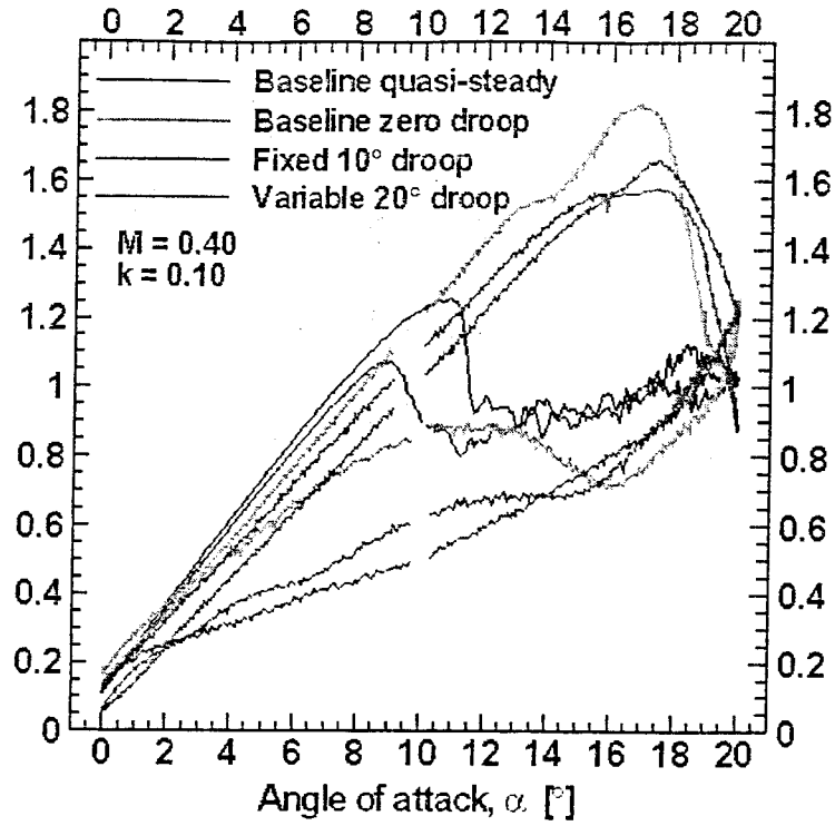
Fig. 17: Lift coefficient integrated from measured pressure distributions.
