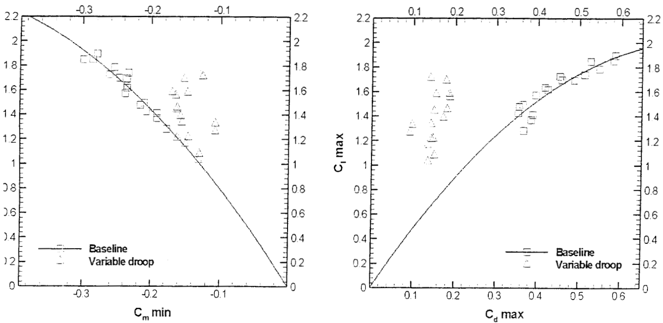
Fig. 20: Bousman's dynamic stall function (Ref. 15) for the VR-12 with and without variable droop (mean angle 10 deg, k=0 to 0.1, and M=0.2 to 0.4).
