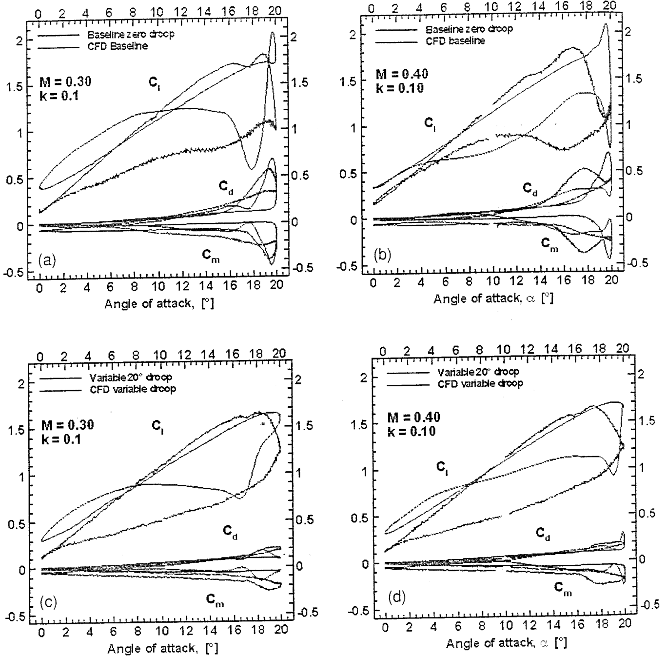
Fig. 4: CFD results compared to measurements.
