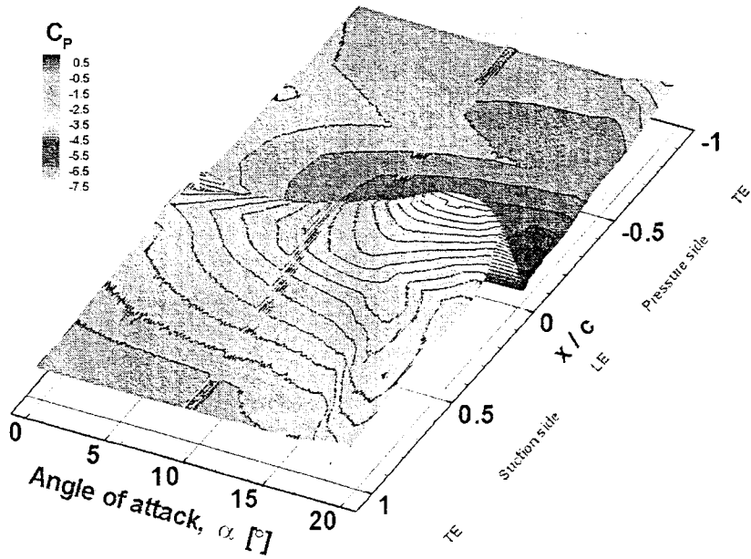
Fig. 16: Pressure contours during the upstroke
