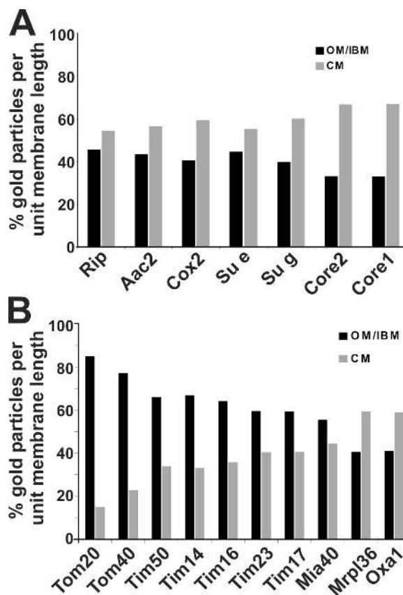
Figure 3. Subcompartmental organization of mitochondrial proteins. Quantification of the distribution of mitochondrial proteins in wild-type cells under respiratory growth conditions was performed as described in Figs. 1 and 2 and Materials and methods. (A) Proteins involved in OXPHOS. (B) Proteins involved in the insertion of nuclear- and mitochondrial-encoded proteins.
