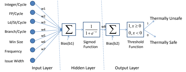
Figure 3: Neural network classifier architecture.
