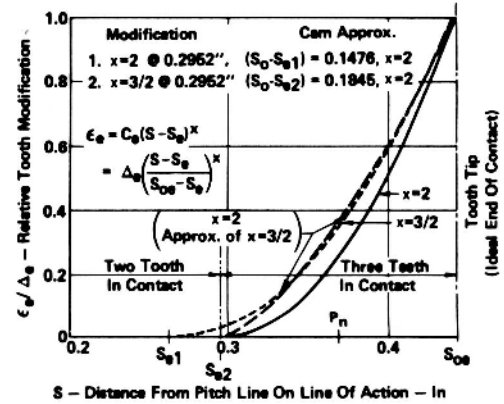
Figure 5. - Approximation of tooth profile modifications for LCRG.
