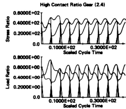
Figure 13. - Effect of tooth errors on dynamic tooth loads and stressing of HCRG. M = 0.001 \text{ lb}\cdot\text{sec}^2/\text{in.} ; u = 0.02 ; N = 10\,000 \text{ rpm} .
