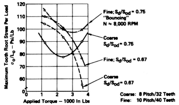
Figure 12. - Effect of applied torque on dynamic tooth stressing of HCRG. M = 0.001 \text{ lb}\cdot\text{sec}^2/\text{in.} ; \xi = 0.02 ; N = 9500 \text{ rpm} .
