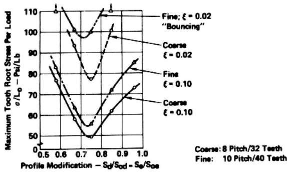
Figure 11. - Effect of profile modification length on dynamic tooth stressing of coarse and fine HCRG. M = 0.001 \text{ lb}\cdot\text{sec}^2/\text{in.} ; N = 9500 \text{ rpm} ; T = 2400 \text{ in}\cdot\text{lb} .
