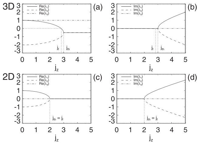
FIG. 3. Real and imaginary parts of the central null point/line eigenvalues as a function of current at the null ( j_z ) throughout the primary bifurcation in 2D ( \kappa=0 ) and 3D ( \kappa=1 ). Based on the model in Eq. (1); in both cases x_T = y_T = B_0 = L_0 = 1 .
