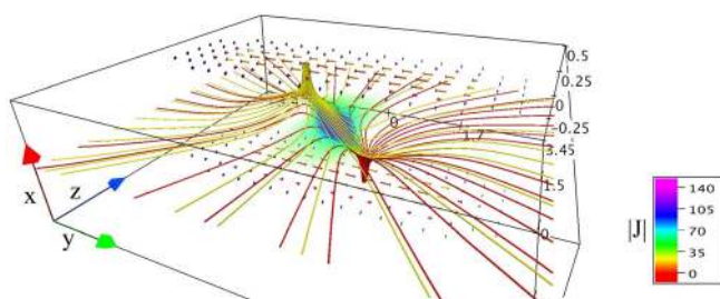
FIG. 1. The magnetic field in the simulation at t=9 (corresponding to the end of stage I), depicting the setup of the experiment. Arrows show the tangential driving velocities applied on the x boundaries, volume shading shows the current density, and red and yellow field lines show the 3D null point magnetic field structure.
