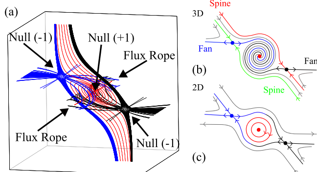
FIG. 2. Model of the field structure immediately after the primary bifurcation. (a) The 3D field structure; (b) schematic of the field in the xy -plane; (c) schematic of the magnetic topology following a symmetric pitchfork bifurcation in 2D, for comparison. When the field is 3D, \partial B_z / \partial z \neq 0 lending the field an open configuration, see text for details.
