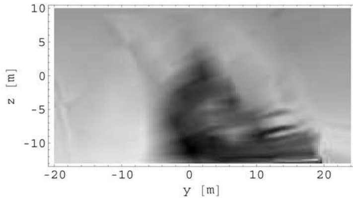
Figure 3-9 Sphere Scan of a downstream wake. Darker areas are lower wind speed, and the LiDAR continuously scans the wake and the velocity regime outside the wake. This plot is based on approximately 1 second of measurements. The focus distance is 58 m. From [15].
