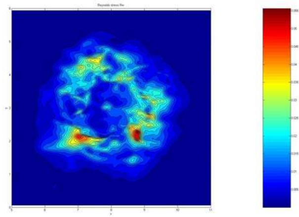
Figure 2-26 Reynolds stresses R(w,w) . Minimum value equal to 0; Maximum value equal to 5.5%.
