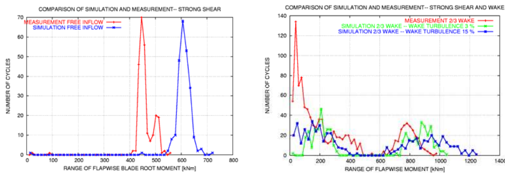
Figure 3-18 Rainflow counting on the flapwise moment. To the left the free inflow situation is shown, and to the right is shown the 2/3 wake case and the influence of increasing the wake turbulence.
