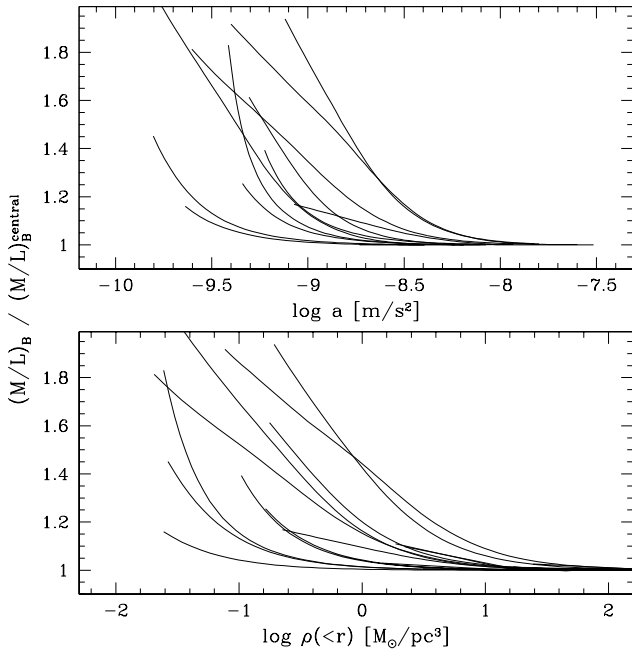
FIG. 19.— Top : B -band M/L_B , normalized by the central M/L_B , vs. the gravitational acceleration v^2/r for all galaxies from the EK subsample. The “bending upward” occurs at accelerations a \sim 10^{-9} \text{ m s}^{-2} , a factor of 10 higher than typical in spiral galaxies. Bottom : Normalized M/L_B vs. mean interior density.
