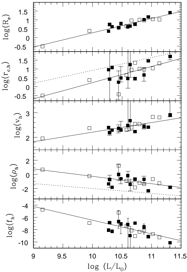
FIG. 18.—From top to bottom: effective radius in kpc vs. total luminosity in solar units; halo core radius in kpc; halo velocity in \text{km s}^{-1} ; central halo density in M_{\odot} \text{pc}^{-3} ; and central halo phase-space density in M_{\odot} \text{pc}^{-3} (\text{km s}^{-1})^{-3} , all referring to the “best” models selected by K + 2000 from the middle of the respective confidence range for all sample galaxies. Symbols are as in Fig. 5. The solid lines show the least-squares fits. Dotted lines show the corresponding relations for spiral galaxies given in the text.
