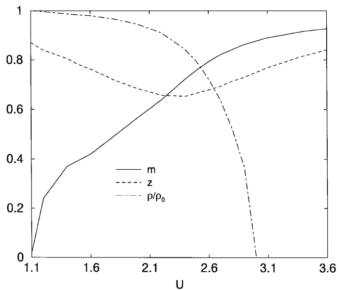
FIG. 1. The magnetization m , z and the normalized density of states at the Fermi level \rho(0)/\rho_0(0) versus U for t_2/t_1 = 0.57 ( \alpha = 0.25 ) with U_{MIT} = 3.0t .
