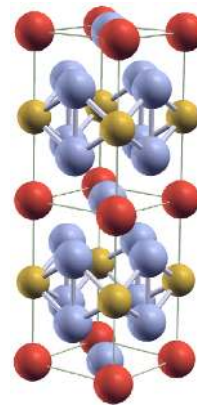
FIG. 12: Crystal structure of CeXIn_5 . Red, yellow and gray spheres correspond to Ce, X , and In atoms, respectively.
