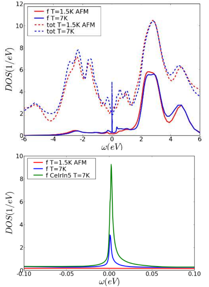
FIG. 18: Total and partial Ce- 4f density of states for Rh115 below and above the AFM transition. Above the Neel temperature, there is a signature of Kondo effect, which partially screens magnetic moment at elevated temperatures, even though the system develops the long range order below 3 K. The quasiparticle peak is however much smaller than the same peak in CeIrIn 5 material. Once in the ordered state, the quasiparticle peak disappears.
