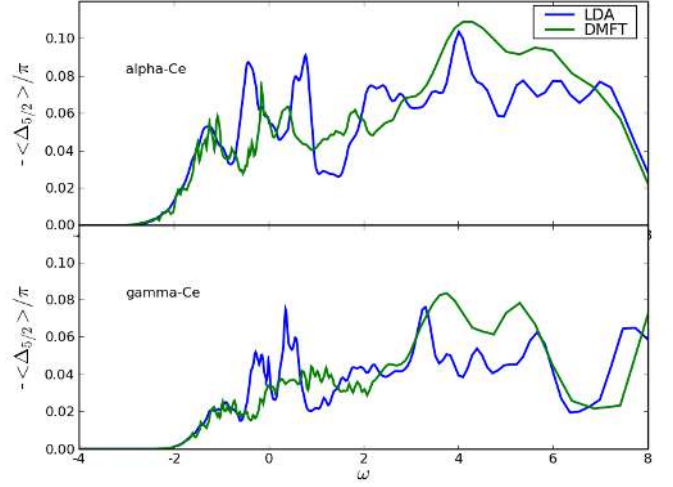
FIG. 10: The hybridization function of the j_z = 5/2 subshell within LDA and within DMFT in both phases.
