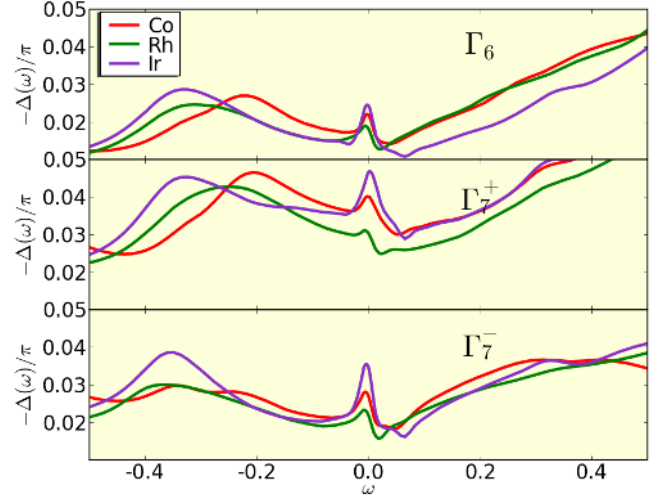
FIG. 16: The frequency dependence of the three most important hybridization functions \Delta''(\omega)/\pi in all three 115 compounds: CeCoIn 5 , CeRhIn 5 and, CeIrIn 5 . The frequency is in units of eV.
