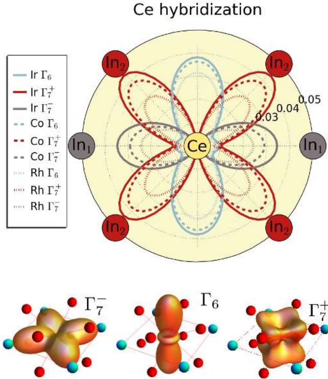
FIG. 15: The Ce-4 f Weiss field hybridization function |\Delta''|/\pi decomposed into crystal field components of tetragonal field. All quantities are in units of eV. The upper plot shows the 2D projection of the three relevant orbitals, while the lower panel shows their 3D shapes (blue dots mark the position of the in-plane In atoms, while the red dots the position of the out-of-plane In atoms). The radial extend of the orbitals in the polar plot of the upper panel is proportional to the value |\Delta''|/\pi at zero frequency. The full/dashed/dotted lines correspond to CeIrIn 5 /CeCoIn 5 /CeRhIn 5 . While all three components of hybridization \Gamma_7^- , \Gamma_7^+ , and \Gamma_6 , are largest (smallest) in CeIrIn 5 (CeRhIn 5 ) compound, \Gamma_7^+ takes the largest value and also changes more than the other two components.
