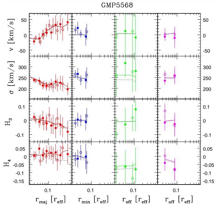
Figure A3. As Fig. A1, but for GMP5568/NGC 4816. Green/third column: offset to major-axis r_{\text{eff}}/4 ; magenta/fourth column: offset to major-axis r_{\text{eff}}/20 .
