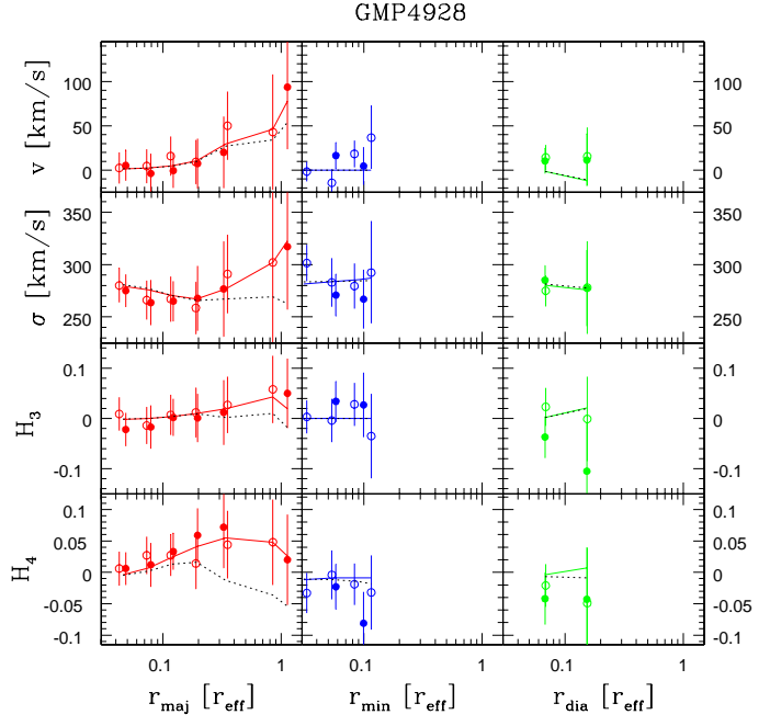
Figure A4. As Fig. A1, but for GMP4928/NGC 4839; green/third column: diagonal axis.
