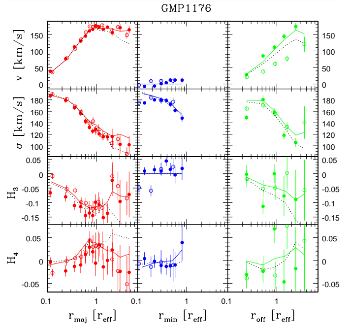
Figure A14. As Fig. A6, but for GMP1176/NGC 4931; green/third column: offset to major-axis r_{\text{eff}}/3 .
