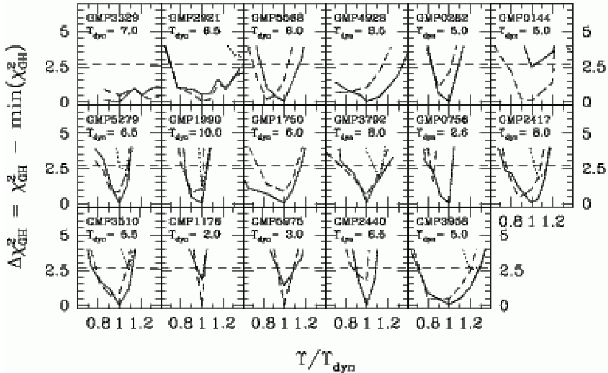
Figure 2. Confidence levels \Delta\chi^2_{\text{GH}} versus \Upsilon (normalised to the best-fit \Upsilon_{\text{dyn}} ). Solid: logarithmic halos; dashed: NFW halos; dotted: mass follows light; horizontal dashed: 90 percent confidence limit. Where a dotted line is missing the self-consistent case is ruled out with more than 95 percent confidence (exception: GMP3329, where the best-fit \Upsilon_{\text{SC}} \approx 1.7 \Upsilon_{\text{dyn}} is outside the plotted region). From top-left to bottom-right galaxies are arranged in order of decreasing total mass inside r_{\text{eff}} .
