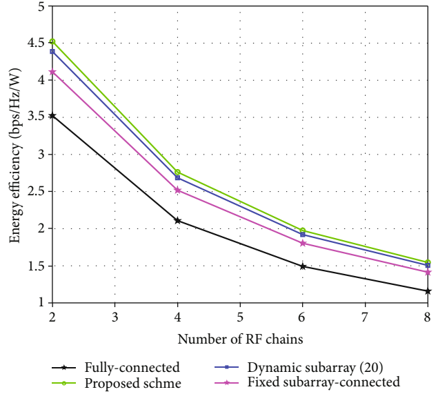
FIGURE 6: Energy efficiency comparison against the numbers of RF chains, where N_T = 128 , SNR = 0 dB, N_R = 2 , and K = 2 .
