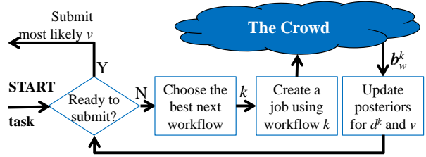
Figure 2: AGENTHUNT’s decisions when executing a task.
