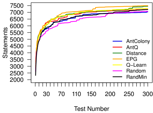
Figure 6.6: TerpWord Cov. Increase
