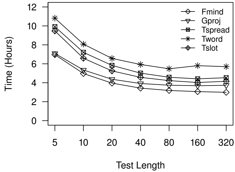
Figure 4.4: Run Time
