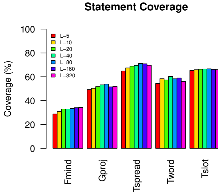
Figure 4.1: Statement Coverage
