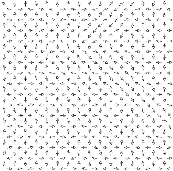
FIG. 1: A 16 \times 16 model system with d = k_1 = k_3 = 0.1 , in a metastable state at temperature k_B T / \varepsilon = 0.025 , from a hysteresis scan (this is a state at h_{\text{ext}} = 0 ). Most of the system is locally close to the Z = +1 ground state. The upper right hand corner is locally near the Z = -1 ground state, and there is a bent domain wall connecting the two regions. For interior charge sites (junction points of four islands), there happens to be no discrete monopole charges present: all q_k = 0 and the discrete \rho_m = 0 .
