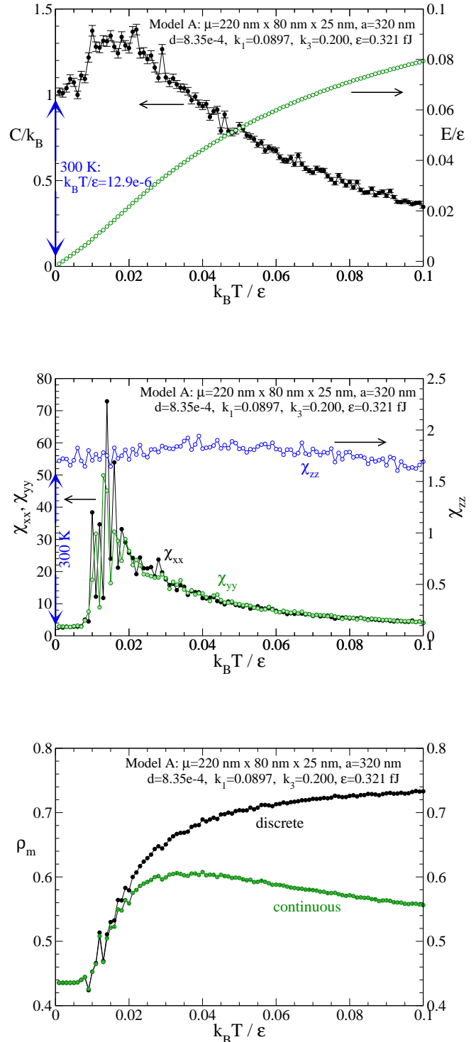
FIG. 2: (Model A) For a 16 \times 16 grid of particles as used in Wang et al. with indicated parameters, (a) the internal energy and specific heat per site versus scaled temperature; (b) the components of the magnetic susceptibility at zero external field; (c) The monopole density, Eq. (8) as determined from discrete and continuous charge definitions, Eqs. (6) and (7). The vertical arrows very near k_B T / \epsilon = 0 show room temperature: it is essentially inaccessible in this dynamics.
