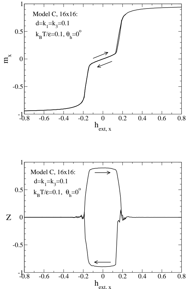
FIG. 5: (Model C) With D = L_1 = K_3 = \frac{1}{10}\epsilon , at temperature k_B T = \frac{1}{10}\epsilon , (a) the averaged magnetization per site versus external magnetic field h_{\text{ext}} applied along the x -axis; (b) the order parameter Z versus h_{\text{ext}} . The field strength was initially set at h_{\text{ext}} = 0.8 , and scanned to h_{\text{ext}} = -0.8 , then back to the starting value as in a hysteresis loop calculation.
