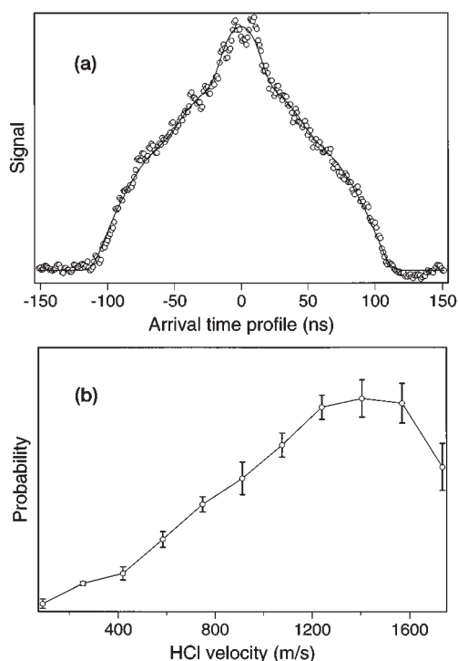
FIG. 3. (a) Core-extracted ion-arrival profile for HCl ( v=0, J=1 ), along with the calculated best fit function. Spatial anisotropy has been removed by forming a composite profile from the isotropic sum, I_{\text{iso}} = I_{\text{par}} + 2I_{\text{perp}} of profiles measured with the photolysis polarization parallel and perpendicular to the TOF axis. (b) Speed distribution of HCl ( v=0, J=1 ) resulting from a maximum-entropy analysis that fits the arrival profile to a combination of instrumental basis functions. Error bars represent 1\sigma statistical deviations of replicate measurements.
