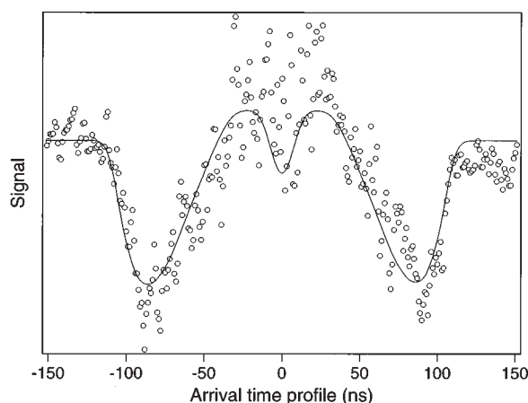
FIG. 5. Core-extracted ion-arrival profile for HCl ( v=0, J=1 ). This profile is a composite that contains product spatial anisotropy information; the profile is generated as twice the anisotropic difference of experimental profiles measured with the photolysis polarization parallel and perpendicular to the TOF axis, I_{\text{aniso}} = 2(I_{\text{par}} - I_{\text{perp}}) . The solid line shows the fit to the data as a sum of instrumental basis functions obtained through a least-squares fitting algorithm.
