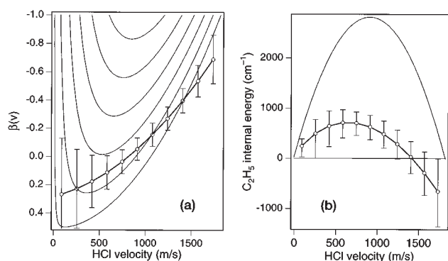
FIG. 8. (a) HCl product spatial anisotropy as a function of speed, as in Fig. 7, with added contours that indicate the calculated relationship between \beta and v for varying degrees of C 2 H 5 internal excitation. The outermost curve shows the predicted form for \beta(v) assuming no C 2 H 5 internal excitation; inner contours are spaced by 500 cm -1 in ethyl excitation. (b) C 2 H 5 internal energy excitation plotted as a function of HCl velocity. This plot results from a transformation of the data shown in Fig. 8(a), as detailed in the text.
