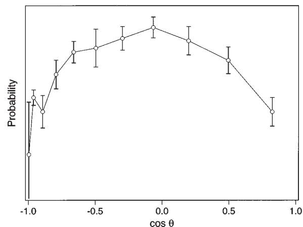
FIG. 4. Differential cross section for the reactive product HCl ( v=0, J=1 ), calculated from the measured speed distribution shown in Fig. 3. The calculation requires an assumption of the \text{C}_2\text{H}_5 internal energy. For this analysis, the ethyl fragment is assumed to take negligible energy into internal modes; this assumption is discussed extensively in the text.
