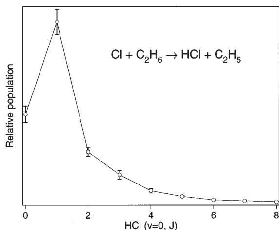
FIG. 1. Plot of the state distribution for the HCl ( v=0, J ) product from the reaction of atomic chlorine with ground-state ethane. Error bars represent 1 \sigma statistical deviations. Relative populations are determined from REMPI spectra as described in the text.
