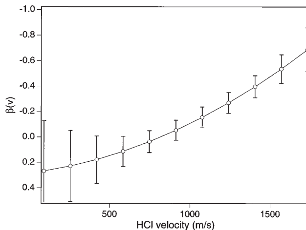
FIG. 7. HCl ( v=0, J=1 ) product spatial anisotropy as a function of speed, \beta(v) , resulting from analysis of the anisotropic time profile shown in Fig. 5. Error bars represent 1\sigma statistical deviations of replicate measurements.
