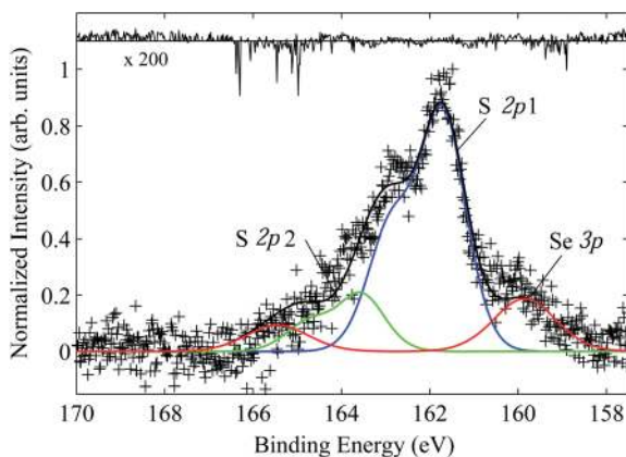
Fig. 15 XPS of the Se 3 p and S 2 p core levels measured with a photon energy of 600 eV. Two species of S 2 p are identified as that associated with the CdS core of the QD (1) and sulfur in the 3-MPA ligand (2).
