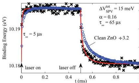
Fig. 13 Binding energy shift of the Zn 3 d core level of the ZnO m -plane surface with PbS QDs chemically attached (black crosses), and of clean ZnO (blue circles, scaled down by a factor of 3.2 for comparison), recorded using a photon energy of 200 eV, during modulation of 3.33 eV (372 nm) CW illumination for a minimum of 10 000 data accumulations. Laser modulation is indicated by arrows. The decay and onset of the pump-induced SPV are fitted using eqn (4) and an analogous decelerating exponential increase respectively (red lines). The decay lifetime, SPV shift and material parameter, \alpha , are reduced when QDs are attached to the surface compared to the clean ZnO case (see text).
