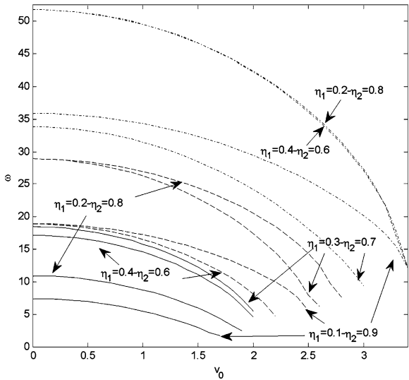
Fig. 6 Variation of the first three modes with axial mean velocity for v_f = 0.2 and for different \eta_1 - \eta_2 locations ( \omega_1 :—, \omega_2 :- - -, \omega_3 :---)
