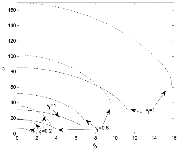
Fig. 2 Variations of the first three modes with axial mean velocity for locations \eta_1 = 0.1 and \eta_2 = 0.9 and for different v_f values ( \omega_1 :—, \omega_2 :---, \omega_3 :-·-)
