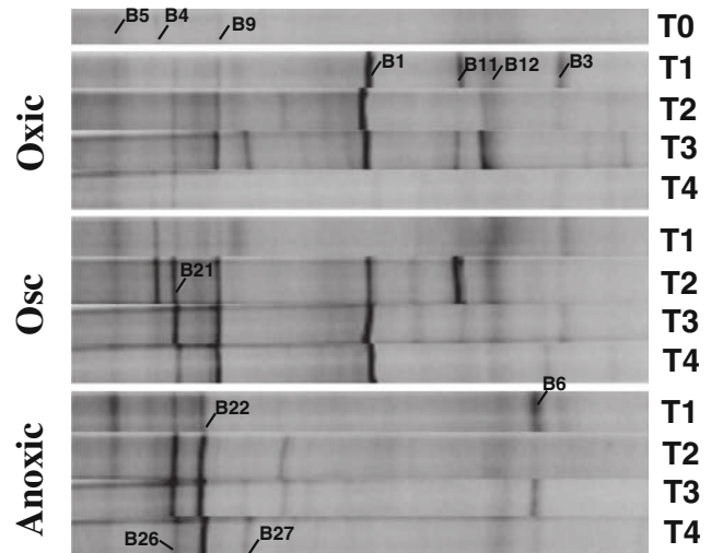
Fig. 5 DGGE patterns of bacterial communities in permanent oxidic (Oxic), permanent anoxic (Anoxic), and in oscillating oxidic-anoxic (Osc) samples for sampling times T0 (initial sampling), T1 (15 days), T2 (30 days), T3 (45 days), and T4 (60 days). Numbers indicate excised and sequenced bands
