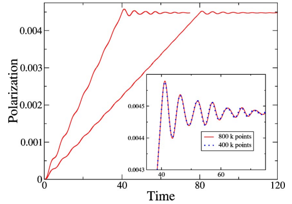
FIG. 5. (Color online) Same as Fig. 4, but now using \mathcal{E}_{\max}=0.05 and 800 k points. Since \mathcal{E}_{\max} is larger than the critical field for this number of k points ( \mathcal{E}_c \sim 0.01 ), no adiabatic curve P_{\text{static}}[\mathcal{E}(t)] is shown. Inset: Comparison of the dynamic polarization for 400 and 800 k points.
