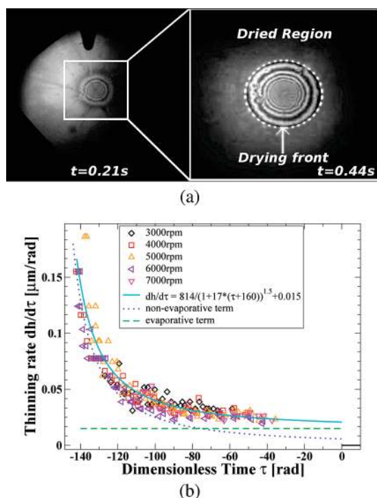
Figure 2. Universality in transient film-thinning dynamics, lighting configuration B. (a) Pattern of alternating rings observed during thinning ( \omega = 5000 rpm = 523.6 rad/s, MEK solvent) at 0.21 and 0.44 s. The last image, t = 0.438 s, shows only the inner region for an enhanced detail of the drying front transition. (b) The derivative of the thickness as a function of time measured from the alternating ring pattern (at radial distances from 1 to 5 mm). A rescaling of time ( \tau = \omega(t - t_{\text{dry}}) ) leads to a collapse of data at all rotation rates. \tau = 0 is the moment when the sample completely dries. The results are well fit by the function in eq 1. Plotting the two terms of the fit (nonevaporative, dotted line; evaporative, dashed line) separately, we see that evaporation likely dominates for \tau > 80 rad.
