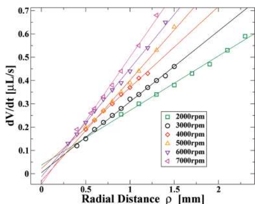
Figure 5. The rate of volume change dV/dt (calculated from experimentally obtained parameters \rho , d\rho/dt , dh/dt , and h ) in the inner region as the drying front advance toward the center.
