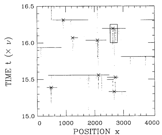
FIG. 10. A sample catalog illustrating the events that take place as a function of position and time. Similar to the sequence of events illustrated in Fig. 4, there the lowest contour (a line segment) marks the first event, and subsequent curves correspond to integration of Eq. (1) forward in time. In this case we forego illustrating the displacement, and instead explicitly plot time on the vertical axis, measured relative to the inverse loading speed, so that values on that axis represent t\nu = \delta U , i.e., the net displacement of initially adjacent points on opposite sides of the fault. A line segment is drawn through all of the blocks that slip during an event, and a cross marks the position of the epicenter of each large event. The clustering of small events in the local minima in Fig. 4 corresponds here to the trails of short line segments, which end at the longer segments, i.e., large events. The box corresponds to a space-time window within which the precursory measures, such as activity or active zone size, which are used in the intermediate-term prediction algorithms are evaluated. The data are taken from a simulation in which \sigma = 0.01 , \alpha = 3 , \xi/a = 10 , and N = 8192 , though only a fraction of the system is shown.
