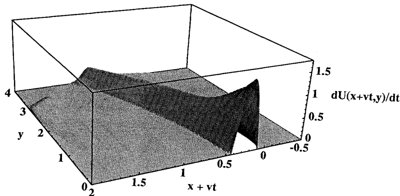
FIG. 9. Snapshot of the slip rate \dot{U}(x+vt, y) in the two-dimensional crustal-plane model, demonstrating the existence of a “self-healing pulse of slip.” The fault lies along the line y=0 , and the snapshot is taken in a comoving frame of velocity -v , where v=1 is the steady-state velocity for this particular pulse. The pulse is propagating to the right along the x+vt axis. The model parameters are \alpha=3.0 , \eta=0.1 . A first-order implicit finite-difference integration has been carried out on a rectangular grid of 250 \times 100 points (with \Delta x=0.01 , \Delta y=0.05 ), although only 80 points are shown in the y direction. The boundaries are free (zero derivative boundary conditions) along all edges except y=0 , where the fault traction is specified by the model. An artificial viscous zone is introduced for y > 4.5 in order to minimize reflections from the back boundary. In this zone, an extra viscous term of the form \eta(y)\nabla^2(\dot{U}) is added to the bulk equation of motion, with \eta(y) growing smoothly from zero.
