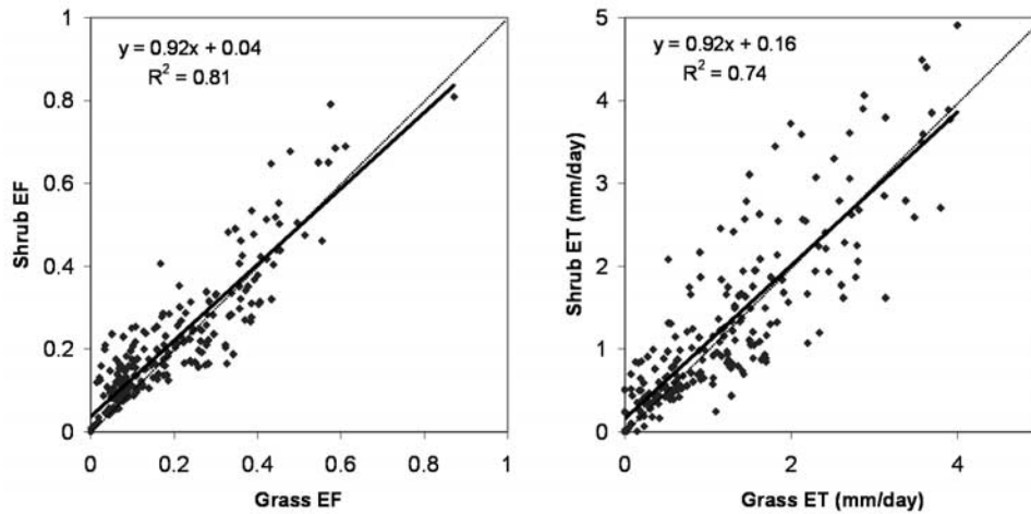
Figure 7. Scatterplot of (a) midday evaporative fraction and (b) daily total evapotranspiration at the grass and shrub sites. Straight line is best fit line via linear regression: dEF_{shrub}/dEF_{grass} = 0.92 and dET_{shrub}/dET_{grass} = 0.92 .
