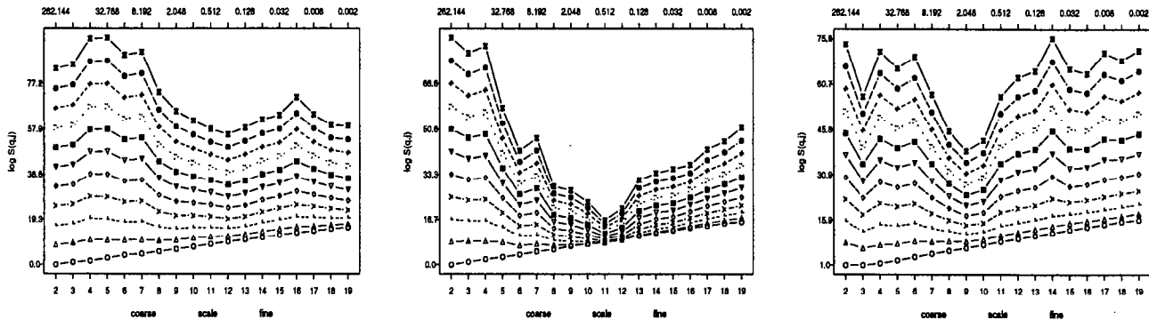
Figure 7: Local scaling analysis: left (FLEXBELL, 400 HIGH-SPEED NODES, PARETO 2); middle (FLEXBELL, 400 MODEM NODES, PARETO 2); right (local scaling plot for measured IP traffic trace DIAL 2, for comparison).
