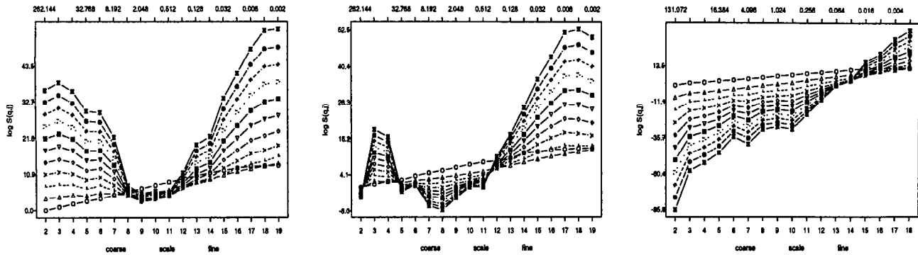
Figure 2: Local scaling analysis plots for three subsets of trace DIAL2: NET1 (left, ISP Web server traffic), NET2 (middle, traffic to news server), NET3 (right, realaudio UDP traffic).
