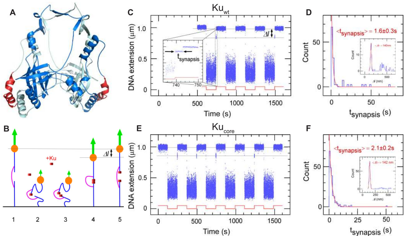
Figure 1. The core structure of bacterial Ku forms short-lived synopsis of blunt DNA ends. (A) 3D model of the bacterial Ku_{wt} homodimer, computed by comparative modelling to the eukaryotic Ku70/80 heterodimer. The red regions highlight the protruding C-terminal arms, which are deleted in the Ku_{core} construct (downstream C-terminal tail of 35 residues predicted as disordered is not represented). (B) Schematic showing the molecular forceps experiment where 1.5 kb (blue) dsDNA segments with blunt ends are joined through a 600 bp dsDNA ‘bridge’ segment (magenta) anchored 59 bases from each end. The blue dsDNA segments are attached to a glass surface (black) and tethered to a magnetic bead (orange), respectively. When extended by a 1.4 pN force (green arrow) by a magnet and in the absence of interacting proteins (1) the DNA construct will have a maximal extension of \sim 1 \mu\text{m} . (2) When the force is lowered to the femtoNewton range the ends can meet (3) and for instance be held together by Ku. This can be seen when (4) the DNA extension does not recover to 1 \mu\text{m} when the force is returned to its initial value: in this case the extension of the construct will be shorter by roughly 140 nm. (5) The construct will return to its initial extension upon disruption of the synapse. (C) Representative time-trace obtained upon force modulation (red) in the presence of Ku_{wt} . Inset shows an expanded view of a rupture event of a single end-to-end synopsis. \Delta l corresponds to the change in DNA extension upon rupture, and t_{synopsis} the duration of the synaptic event. Events are indexed by coordinate pair (\Delta l, t_{synopsis}) . (D) Lifetime distribution for end-specific events is fit to a single-exponential distribution (red), yielding a lifetime of 1.6 \pm 0.3 \text{ s} (SEM, n = 51 ). End-specific events are identified (inset) as having a \Delta l value within three standard deviations of the mean expected amplitude change given bridge mechanics (Gaussian fit in red, \langle \Delta l \rangle = 140 \pm 12 \text{ nm} , SD, n = 99 ). (E, F), As for C and D but for Ku_{core} . The mean lifetime is derived from a single-exponential fit giving a value of 2.1 \pm 0.2 \text{ s} (SEM, n = 212 ). Gaussian fit parameters for amplitude distribution are \langle \Delta l \rangle = 142 \pm 11 \text{ nm} SD, n = 251 ).
