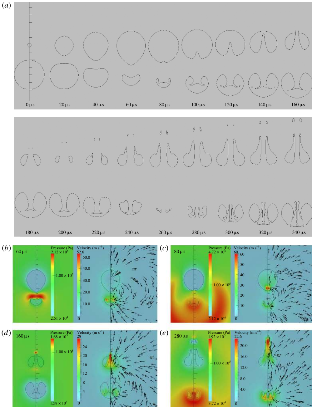
FIGURE 14. Dynamics of an anti-phase bubble pair. Simulation parameters are R_{max1} = 1 mm, R_{max2} = 1.04 mm and \gamma = 1.0 . (a) Bubble shapes; and (b–e) selected frames from the simulation with pressure and velocity fields. To be compared with experimental results from figure 7 with R_{max1} \approx 1 mm and \gamma \approx 1.0 . The numerical peak jet velocities of bubble 1 and bubble 2 are both about 30 \text{ m s}^{-1} .
