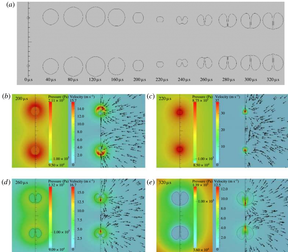
FIGURE 10. Dynamics of an in-phase bubble pair. Simulation parameters are R_{max1,2} = 1.04 mm, \gamma = 2.5 , \tau = 0 and T_{coll} (spherical bubble) = 110 \mu\text{s} . (a) Bubble shapes; and (b–e) selected frames from the simulation with pressure and velocity fields from the first collapse and rebound. Pressure fields (Pa) (note the colour of 1 bar = 10^5 Pa for reference) and flow velocity fields (coloured by velocity magnitude ( \text{m s}^{-1} )) are presented with velocity direction vectors (the arrows) in the right half-space of the simulated area. Each tick of the vertical scale represents 0.5 mm. To be compared with experimental results from figure 4 with the same \gamma = 2.5 . The numerical peak velocity of the jet tip is reached at about 230 \mu\text{s} and amounts to about 25 \text{ m s}^{-1} .
