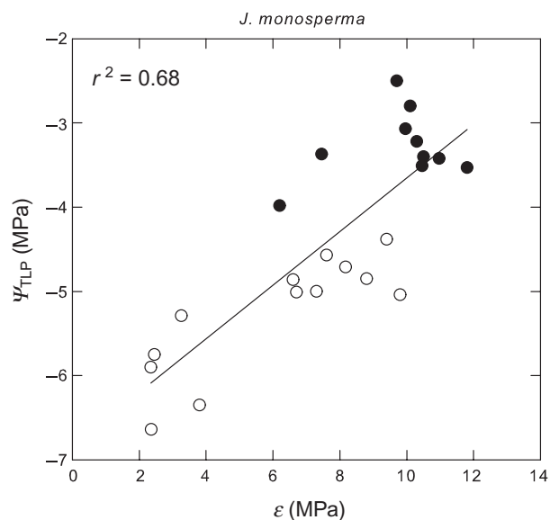
Figure 6. Relationship between the water potential at the turgor loss point ( \Psi_{\text{TLP}} ) and the bulk tissue modulus of elasticity ( \epsilon ) for (○) non-rehydrated and (●) rehydrated J. monosperma shoots excised on different dates during 2012–2013. Data taken from Fig. 3.
