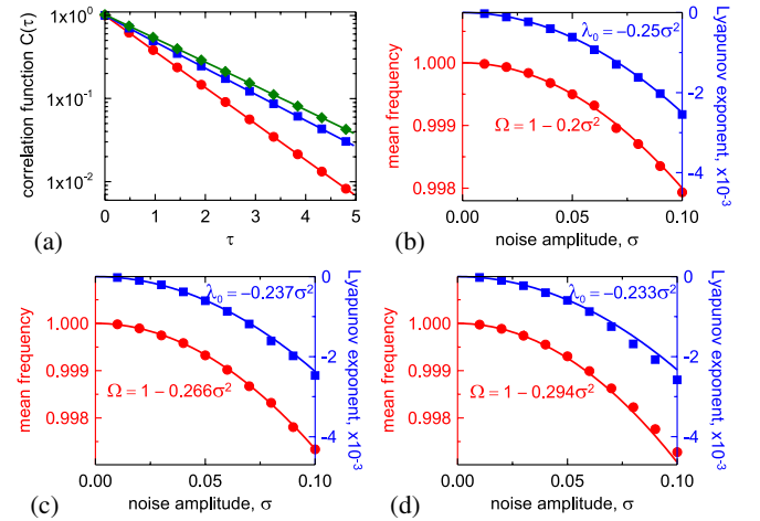
FIG. 1 (color online). Hopf oscillator (12) subject to different noises; here \tau_{\eta} = 1 and \lambda = 2 . (a) Correlation function for Ornstein-Uhlenbeck noise, which is Gaussian, (red circles) and noises with exponential (blue squares) and fractional rational (green diamonds) distributions. (b)–(d) The numerically calculated mean frequency (red circles) and Lyapunov exponent (blue squares) are in good agreement with Eqs. (14) and (15) (solid lines) for OU noise (b) and noises with exponential (c) and fractional rational (d) distributions.
