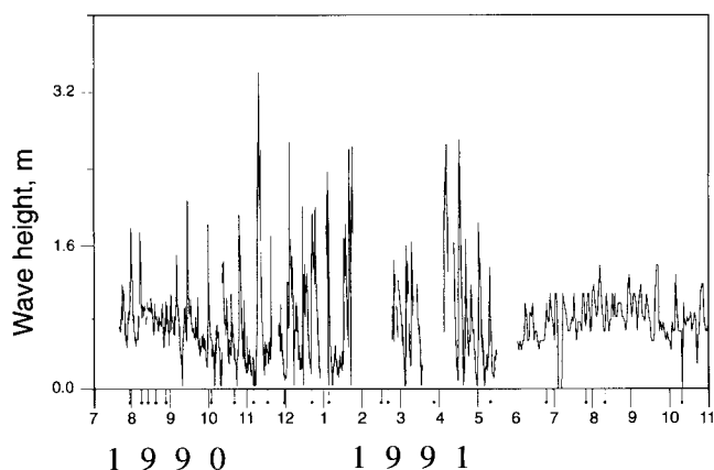
Figure 2. The history of the characteristic wave height measured in the deep water off Hadera, by Givat-Olga, during the study period. The period 7.90–5.91 was calculated by D. Rosen following Komar (1977). The period 6.91–10.91 is based on Titelman (1992). The data were prepared on a common base by D. Rosen, Israel Oceanographic and Limnological Research, Haifa. The months are indicated by numbers and the dots show the days of litter sampling.
