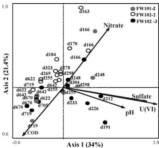
FIG. 6. Canonical correspondence analysis for FW101-2, FW102-2, and FW102-3. Analysis was done using all of the functional genes detected (symbols) and environmental variables (arrows) from FW101-2, FW102-2, and FW102-3. Environmental variables were chosen by automatic selection significance calculated from individual CCA results and variance inflation factors calculated during CCA. Numbers indicate operational days sampled.
