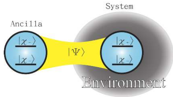
FIG. 4 Schematic illustration of the entanglement measure, which is closely associated with the non-Markovianity measure proposed by Rivas et al. (2010b). A system and an environment isolated copy of it, acting as an ancilla, is considered. Initially, they form a maximally-entangled state. When the system starts to be coupled with its environment (denoted by the gray shadow) it will evolve and the system-ancilla entanglement will be sensitive to the environment coupling. From Chen et al. (2015a).
