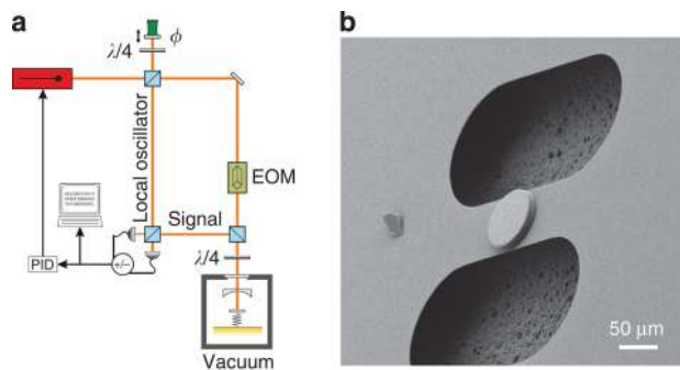
FIG. 1 (a) The experimental set-up consists of a laser, which is split into a signal beam and a local oscillator (LO). The signal beam acquires a phase from the motion of the mechanical resonator, which is detected on two photodiodes after a previous beating of the signal with a strong LO. (b) Scanning electron microscope picture of the tested device. From Groblacher et al. (2015).
