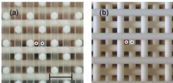
FIG. 2 Side view (a) and top-view (b) photographs of the photonic crystal (scale bar 10nm). The emission dynamics of an emitter was measured considering two different positions: position 1 close to a dielectric rod (left, red dot), and position 2, at a maximum distance from any dielectric rod (right, blue dot). From Hoeppel et al. (2012) .
