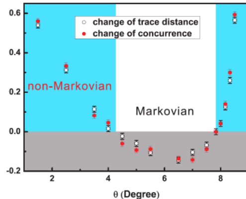
FIG. 3 Changes in the trace distance and the concurrence as functions of the tilting angle \theta . Such an angle determines the structure of the frequency spectrum and, thus, the environmental initial state |\xi\rangle . The positive values in the blue regions give directly the non-Markovianity measure \mathcal{N}(\Lambda) of the process, while the negative values correspond to \mathcal{N}(\Lambda) = 0 , i.e. Markovian dynamics. From Liu et al. (2011) .
