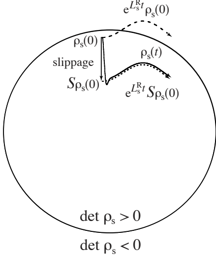
FIG. 5 The space of the reduced matrices \rho_s for a two-level system is divided into the set of admissible density matrices for which \det(\rho_s) \geq 0 so that all the eigenvalues of \rho_s define non-negative probabilities, and the set of non-admissible density matrices for which \det(\rho_s) < 0 . From Gaspard and Nagaoka (1999b).
