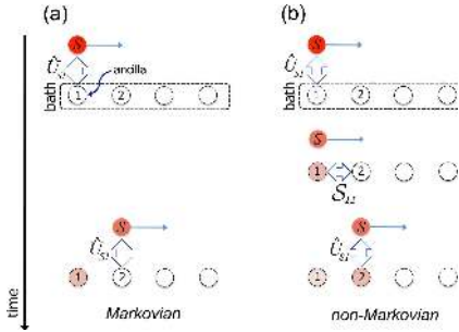
FIG. 6 Schema showing the first steps of the collisional model in the (a) Markovian case, and in the (b) non-Markovian case. In the second case, ancilla-ancilla collisions occur in between system-ancilla collisions. From Ciccarello et al. (2013) .
