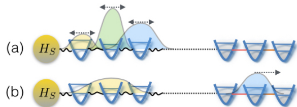
FIG. 7 Partially based on Chin et al. (2011a) . (a) When the system injects excitations into the inhomogeneous part of the chain, some backscattering occurs, reflecting the non-Markovian effects that mainly occur at initial stages of the evolution. (b) At long times the excitations penetrate into the homogeneous region and propagate away from the system irreversibly.
